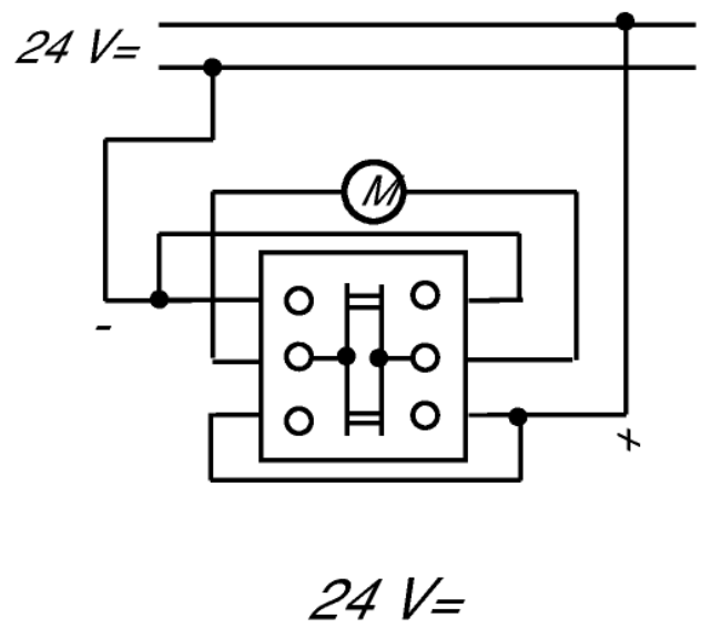
Control of d.c. drive via DP blind switch/push switch 2712 U/ 2722 U
