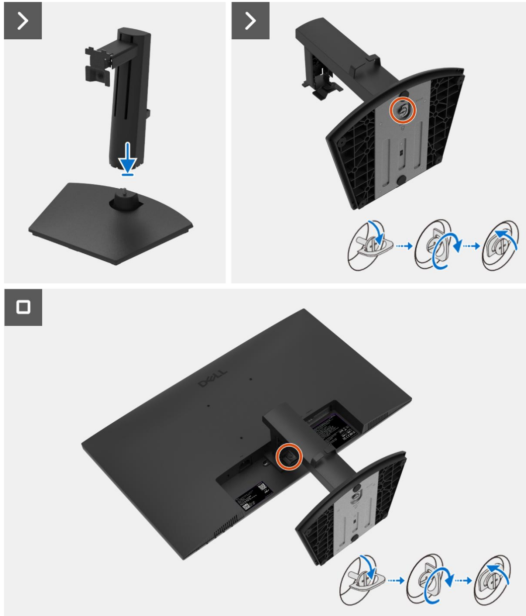
Figure 11. Installing the stand
