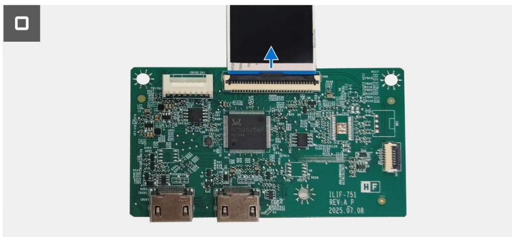
Figure 21. Removing the interface board
