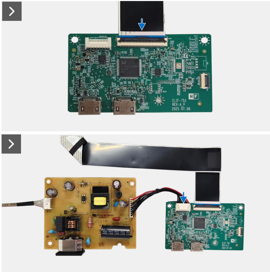
Figure 22. Installing the interface board
