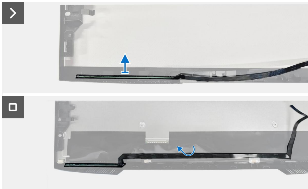
Figure 18. Removing the keypad board
