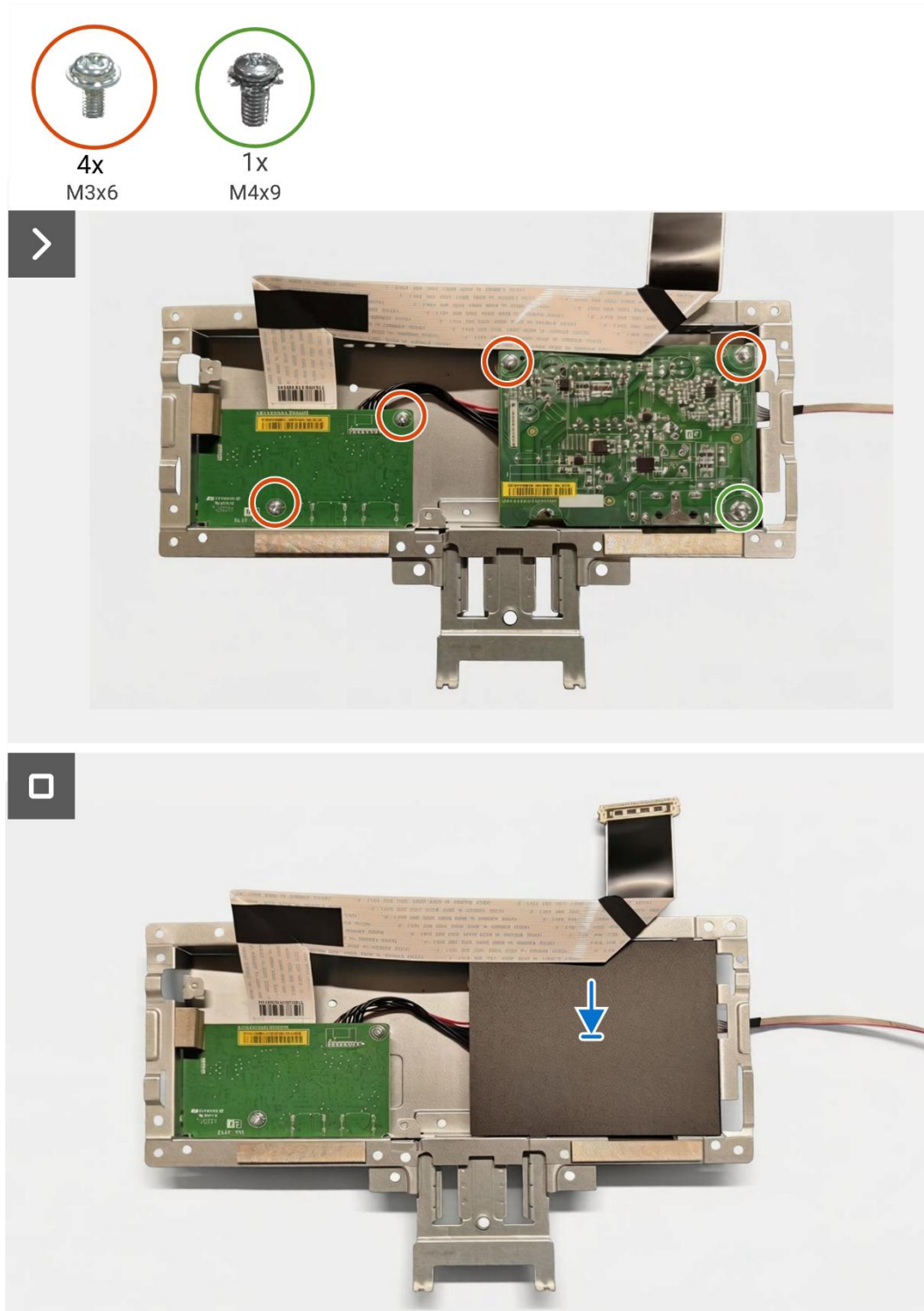
Figure 23. Installing the interface board
