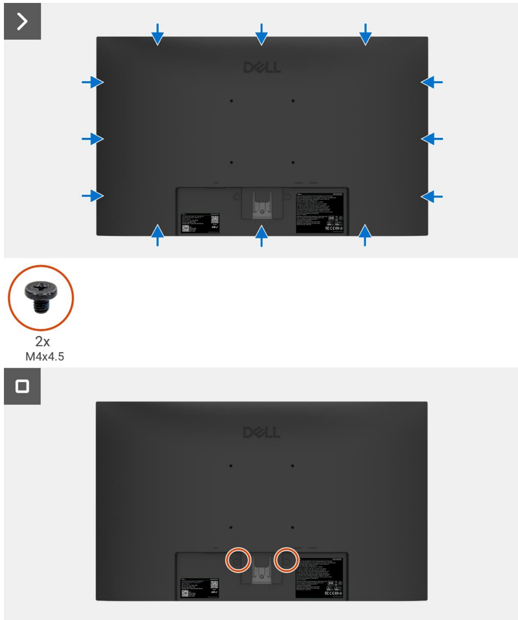
Figure 13. Installing the back cover
