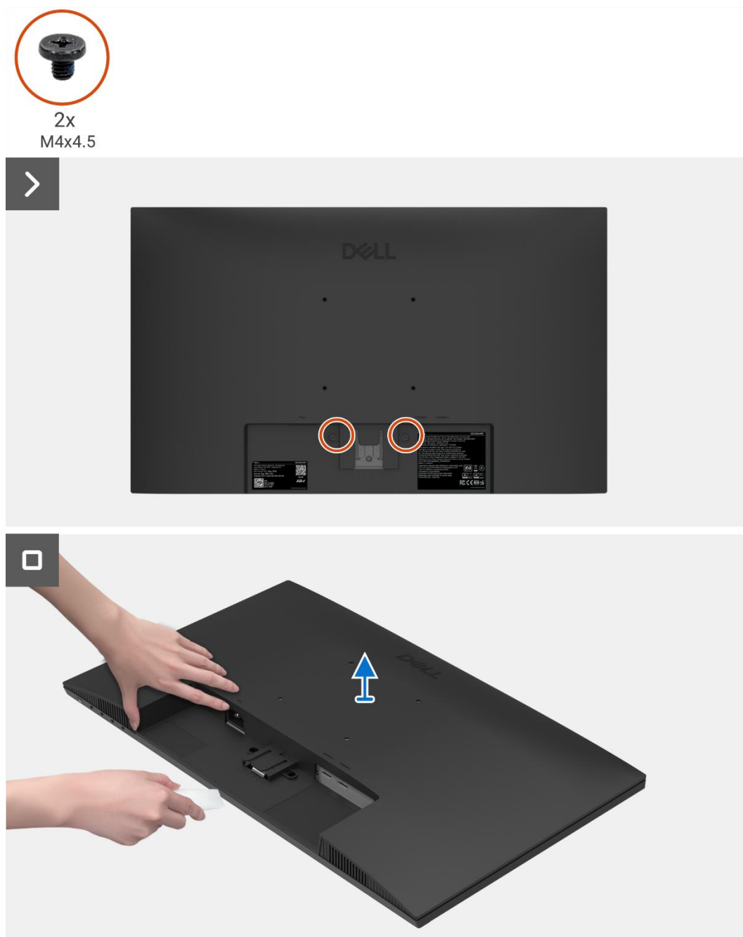
Figure 12. Removing the back cover
