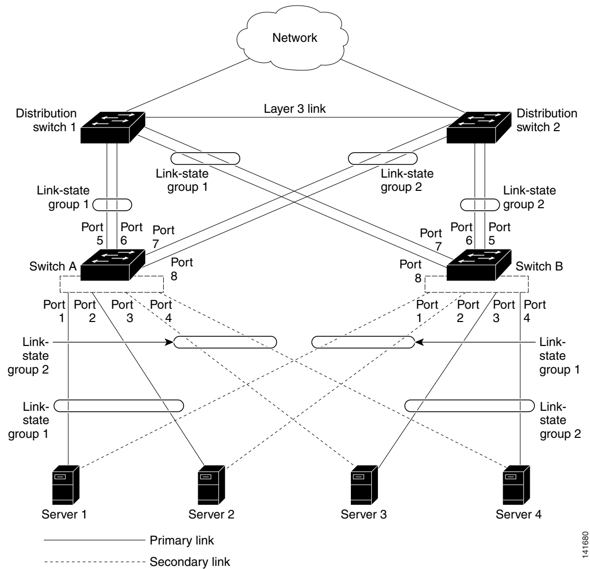
Figure 85 Typical Link State Tracking Configuration
