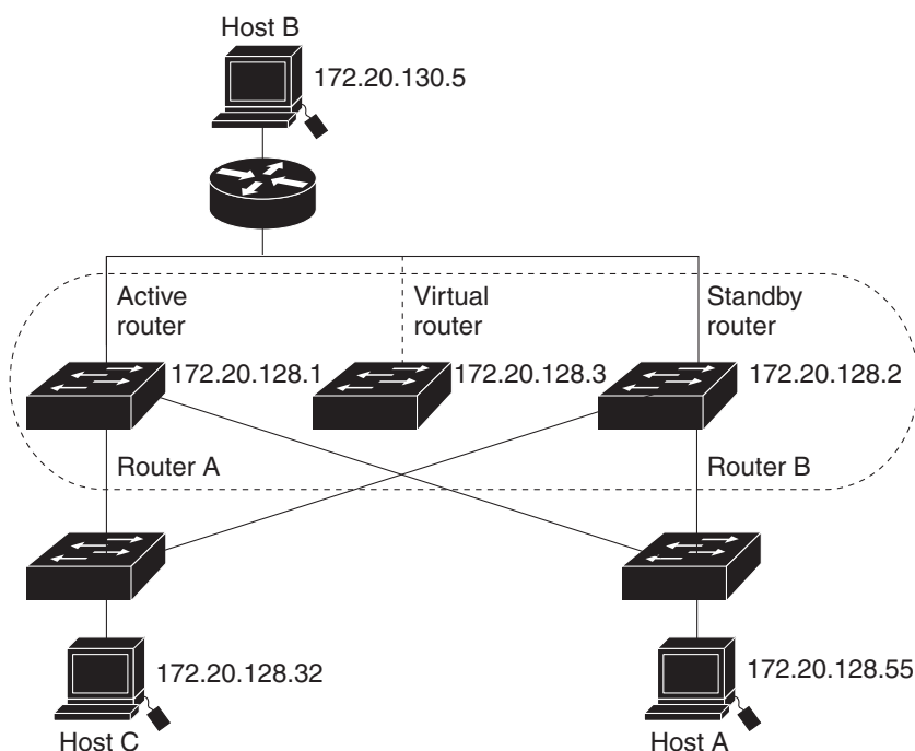
Figure 47-94 Typical HSRP Configuration
