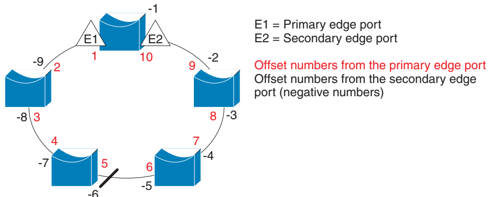
Figure 55 Neighbor Offset Numbers in a Segment
