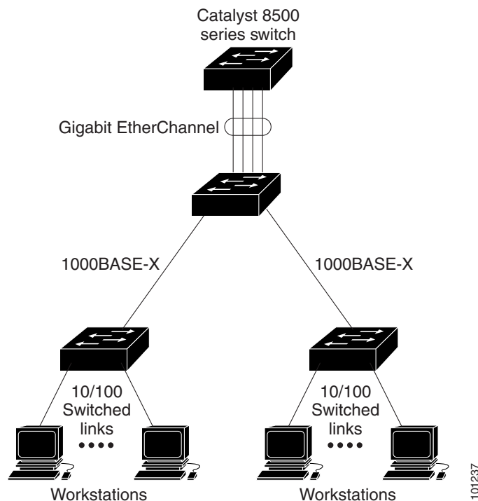
Figure 108 Typical EtherChannel Configuration
