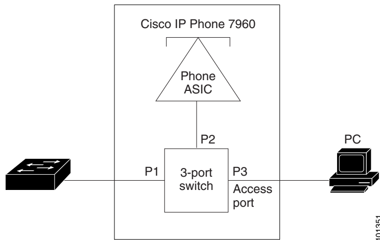
Figure 35 Cisco 7960 IP Phone Connected to a Switch
