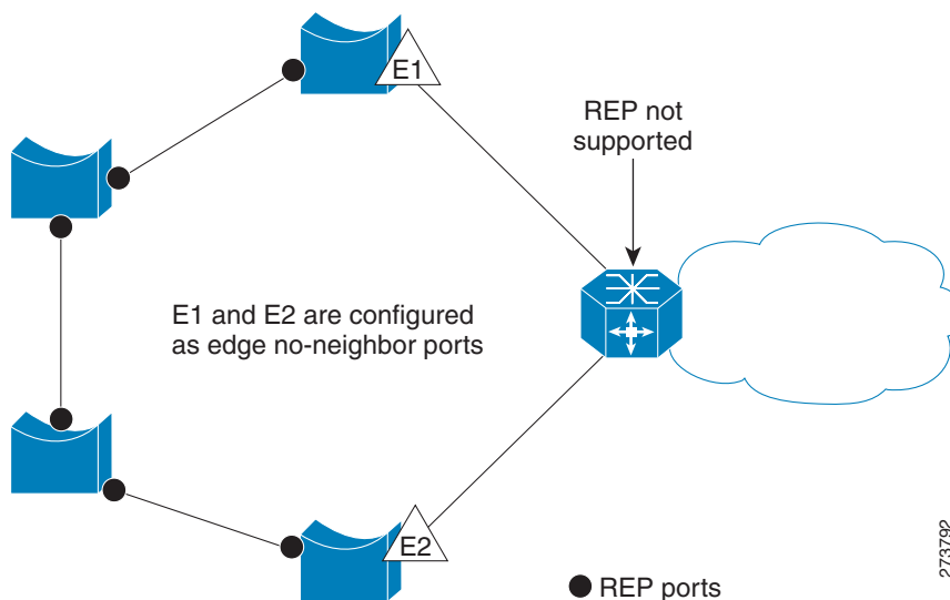
Figure 54 Edge No-Neighbor Ports
