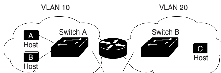
Figure 83 Routing Topology Example
