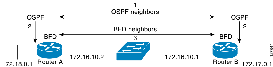
Figure 102 Establishing a BFD Session
