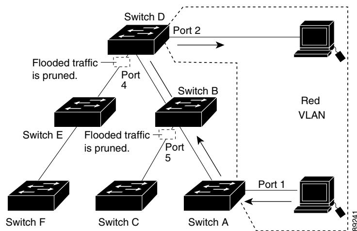
Figure 34 Optimized Flooded Traffic with VTP Pruning
