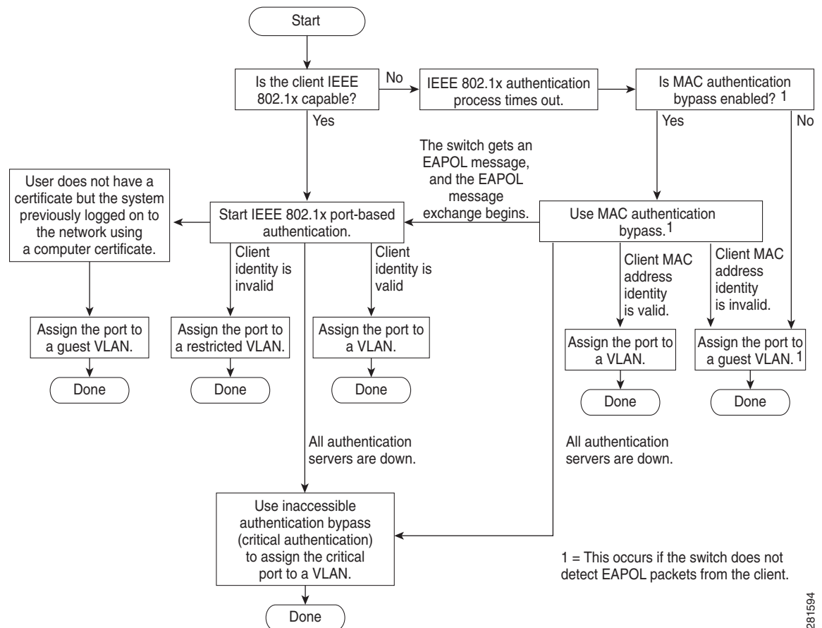
Figure 19 Authentication Flowchart
