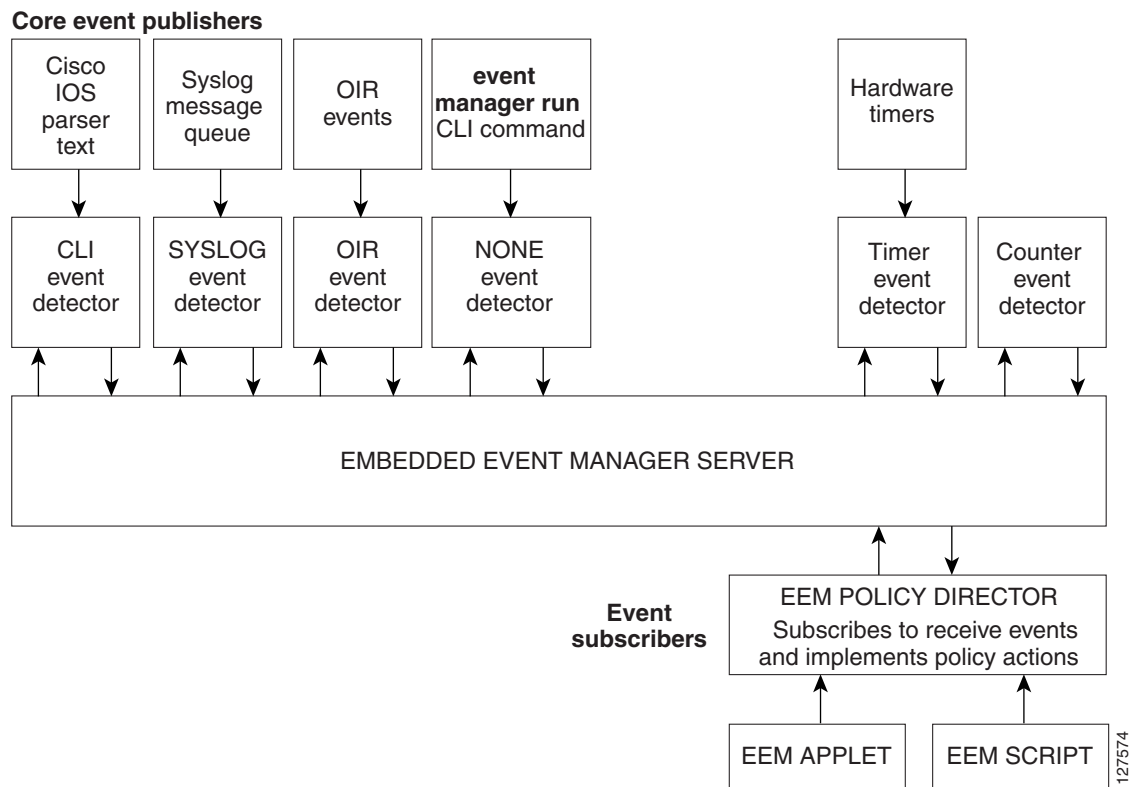
Figure 96 Embedded Event Manager Core Event Detectors
