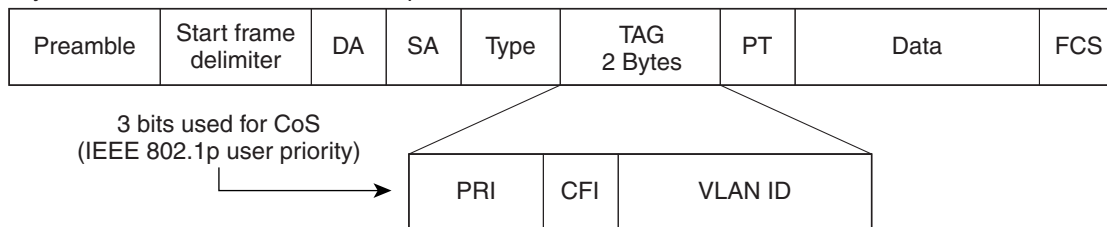
Figure 78 QoS Classification Layers in Frames and Packets
