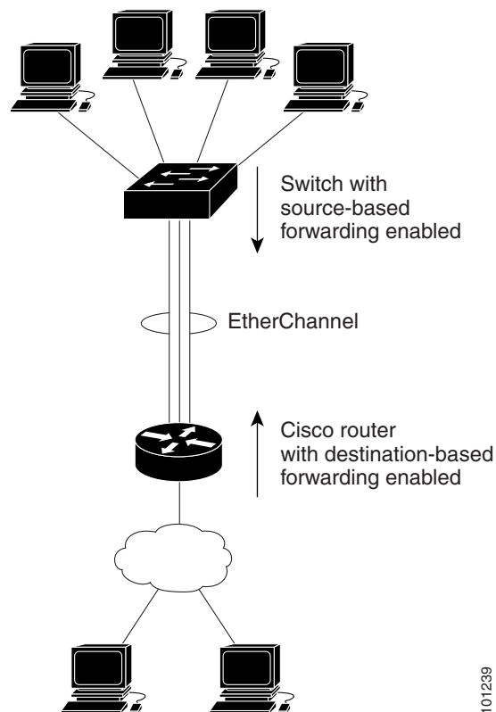
Figure 110 Load Distribution and Forwarding Methods
