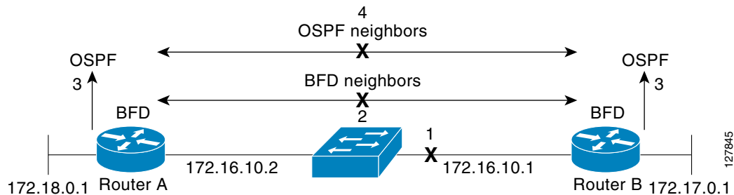
Figure 103 Breaking an OSPF Neighbor Relationship
