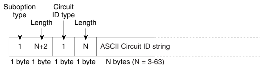
Figure 62 User-Configured Suboption Packet Formats
