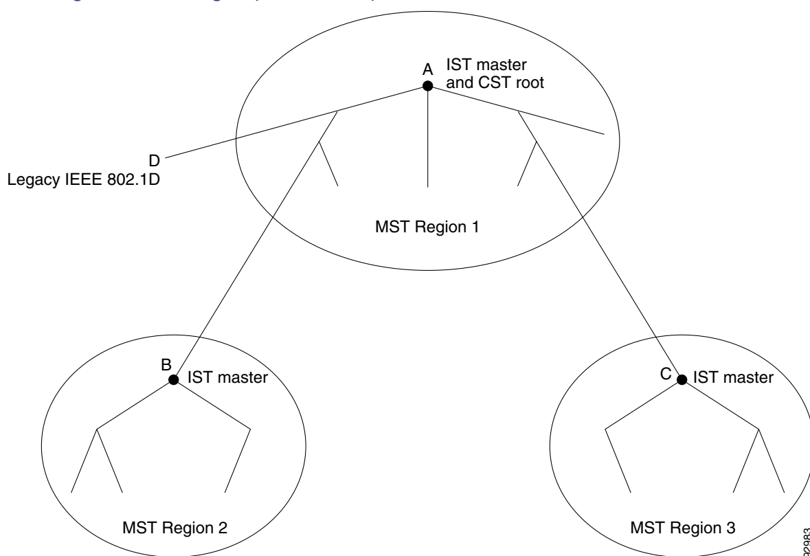
Figure 39 MST Regions, CIST Masters, and CIST Root
