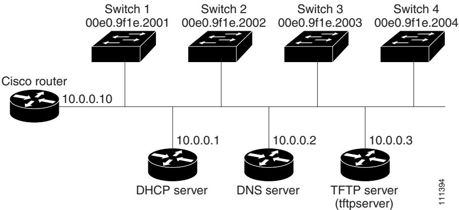
Figure 4 DHCP-Based Autoconfiguration Network Example
