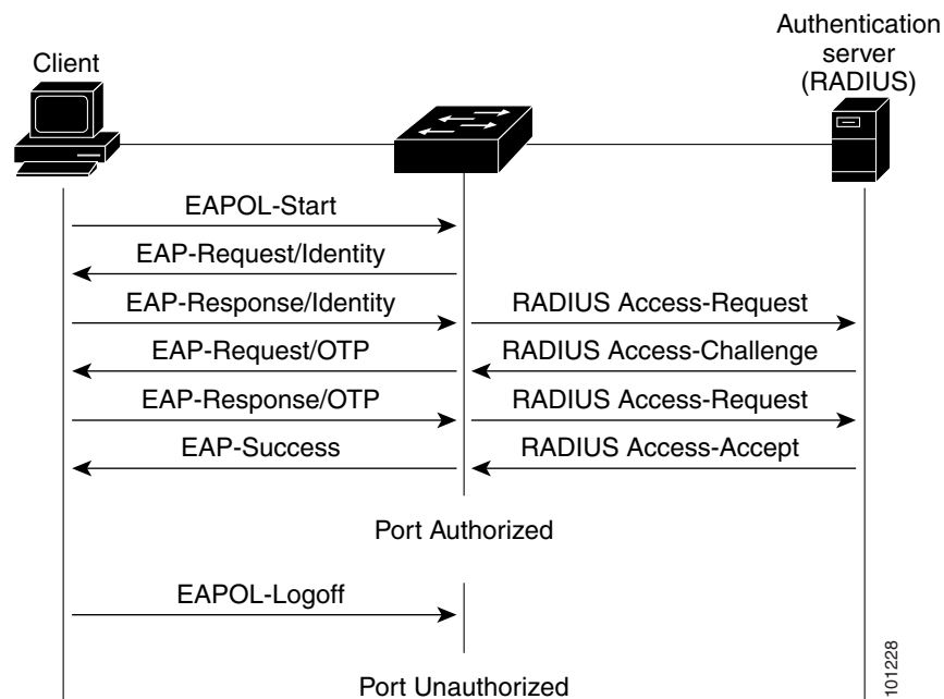
Figure 20 Message Exchange
