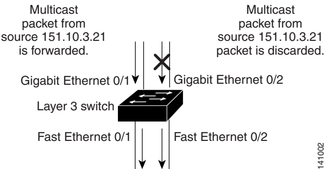
Figure 87 RPF Check
