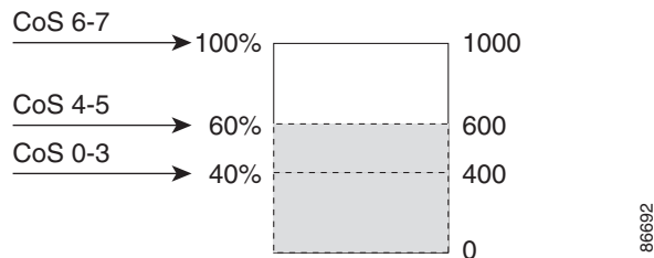
Figure 82 WTD and Queue Operation
