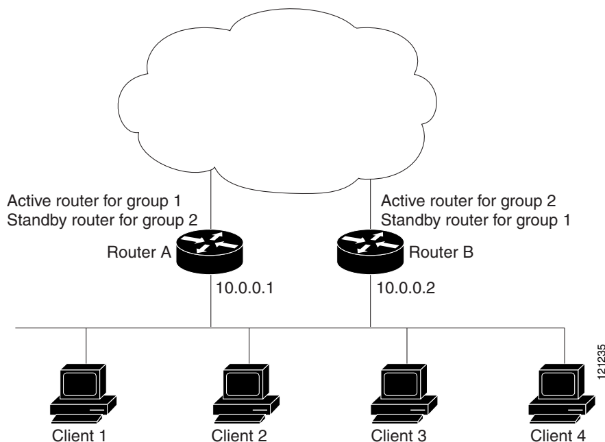
Figure 47-95 MHSRP Load Sharing
