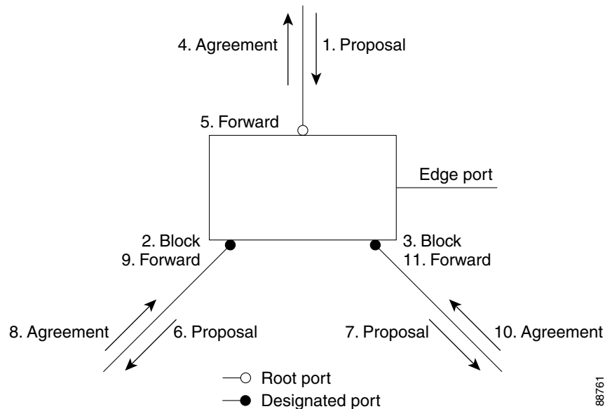
Figure 43 Sequence of Events During Rapid Convergence
