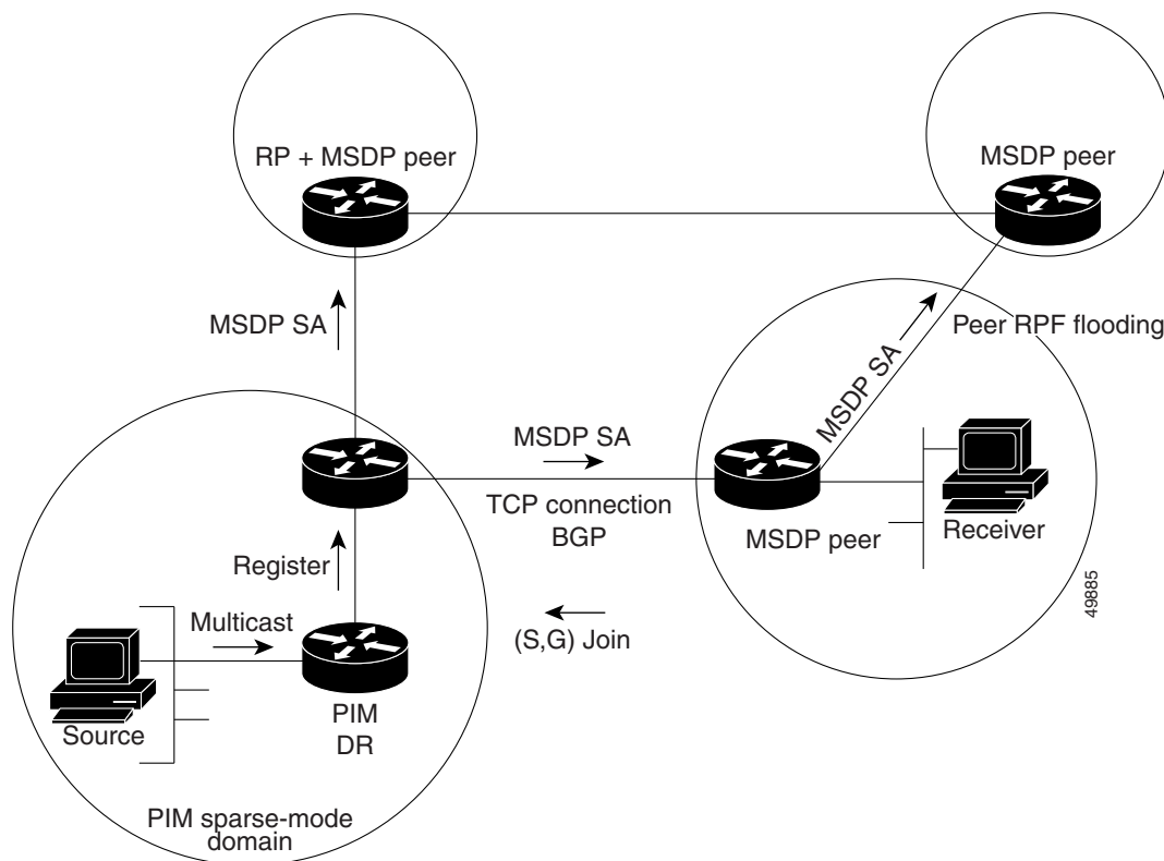
Figure 92 MSDP Running Between RP Peers
