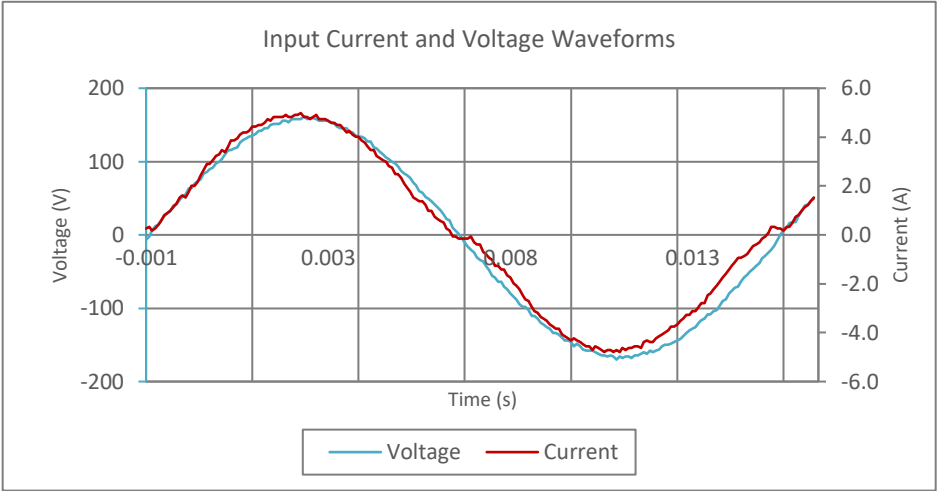
Input AC Current Waveform (ITHD = 7.71%, 50% Load)
