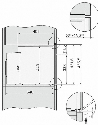
H2840B, H7244B, H7244BP, H7440B, H7440BPX, H7640BP, H7840BP, H7840BPX, Skizze
