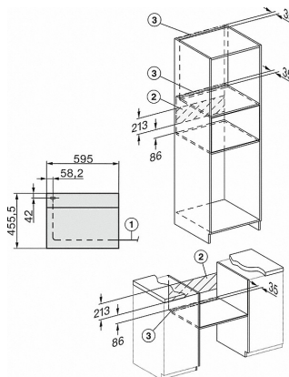
H7x4xB/BP/BPX, H2840B, Skizze
