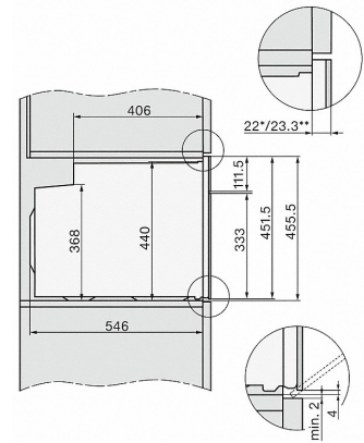
H2840B, H7244B, H7244BP, H7440B, H7440BPX, H7640BP, H7840BP, H7840BPX, Skizze, GB, AUS
