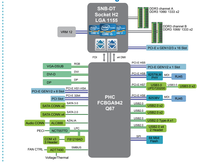
Block Diagram
