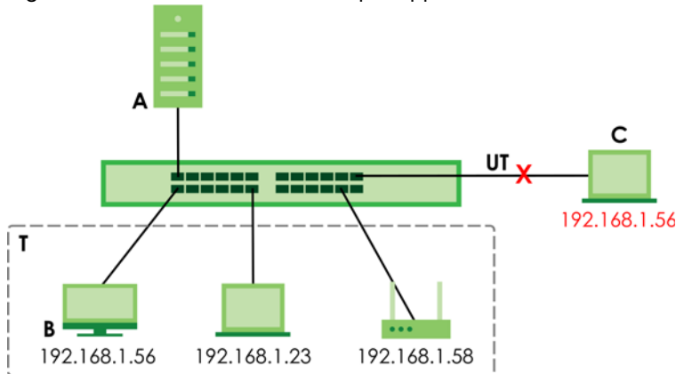
Figure 352 IP Source Guard Example Application
