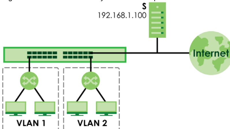
Figure 294 DHCP Smart Relay Network Example
