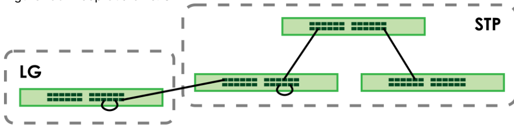
Figure 180 Loop Guard vs. STP
