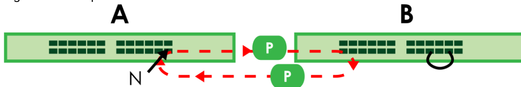
Figure 182 Loop Guard – Probe Packet
