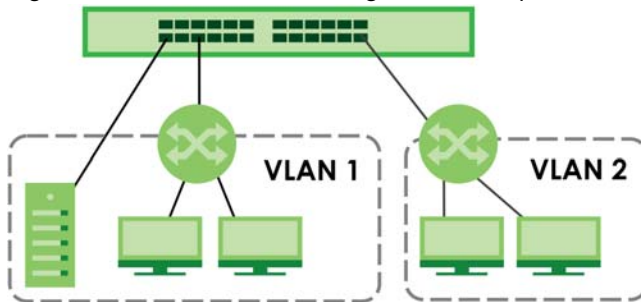
Figure 451 Shared Server Using VLAN Example
