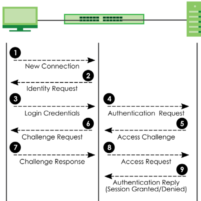
Figure 382 IEEE 802.1x Authentication Process
