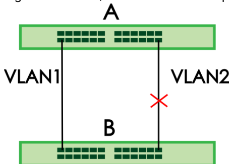
Figure 244 STP/RSTP Network Example
