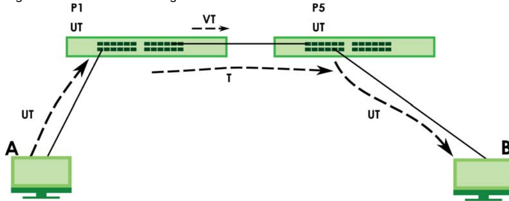
Figure 452 VLAN Forwarding Frame
