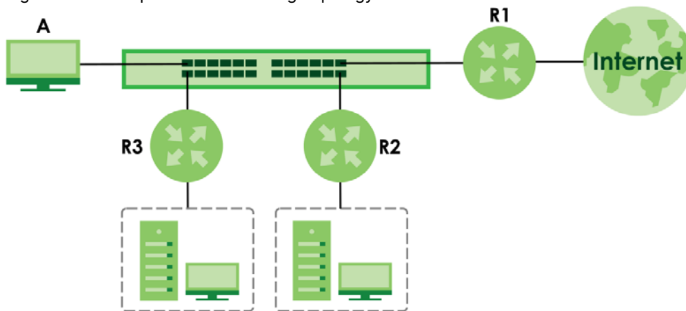
Figure 311 Example of Static Routing Topology
