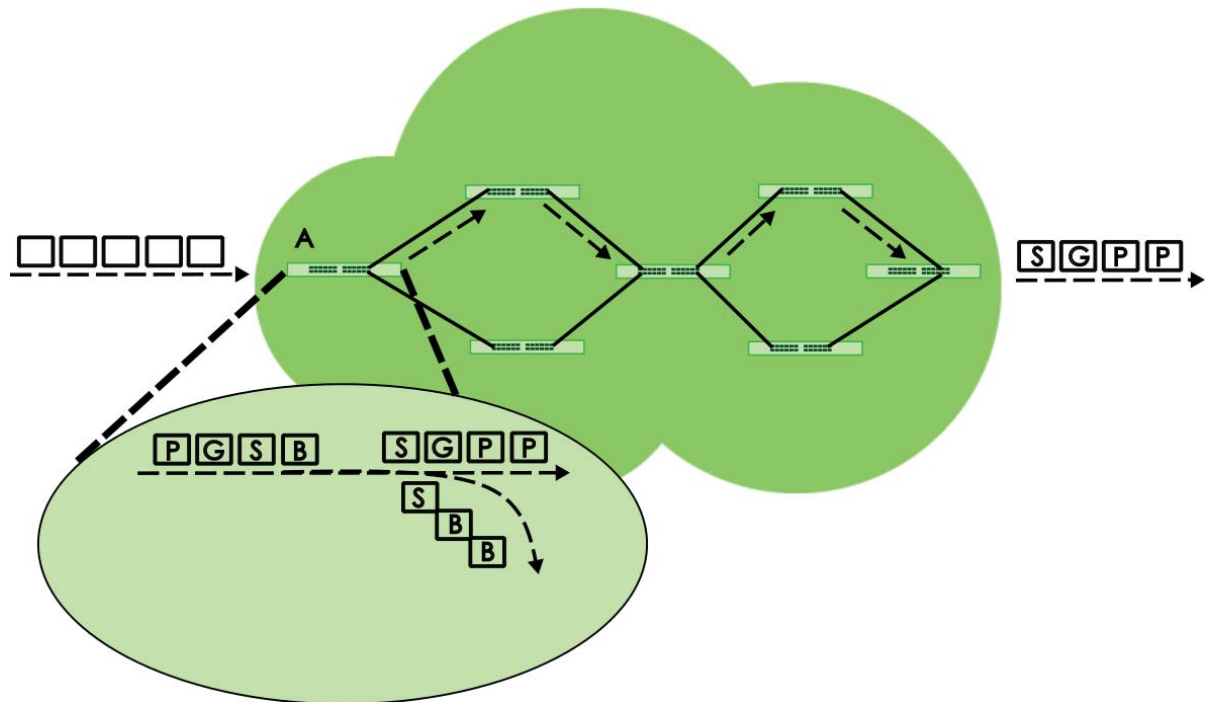
Figure 223 DiffServ Network
