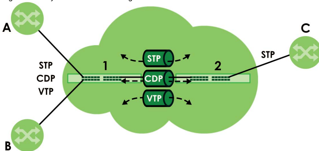
Figure 177 Layer 2 Protocol Tunneling Network Scenario
