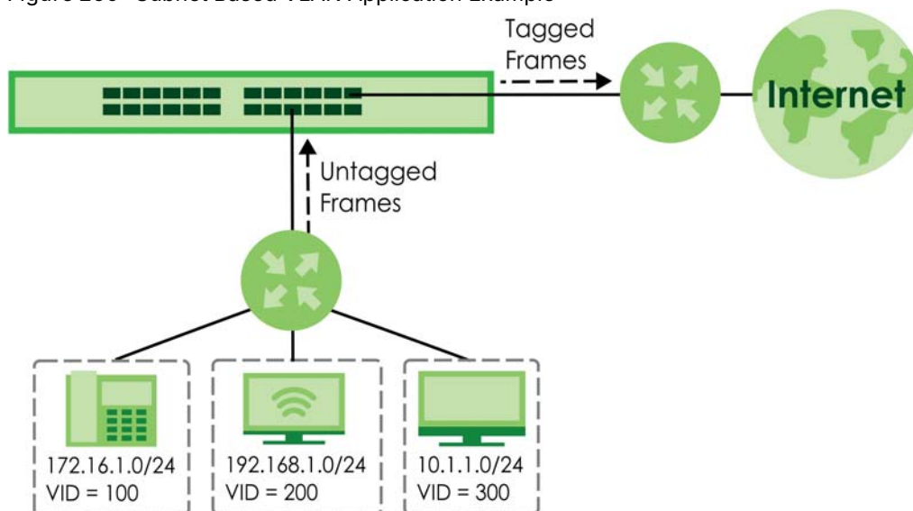
Figure 259 Subnet Based VLAN Application Example
