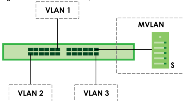
Figure 187 MVR Network Example
