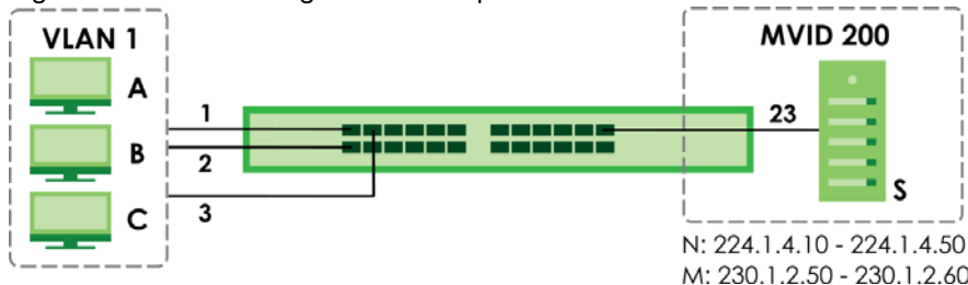
Figure 209 MVR Configuration Example
