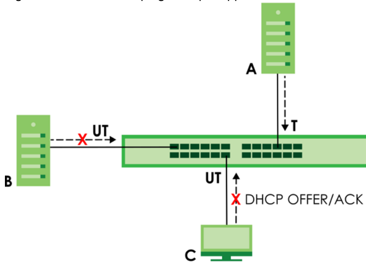
Figure 356 DHCP Snooping Example Application
