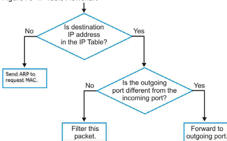
Figure 75 IP Table Flowchart
