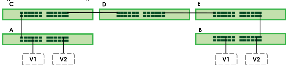
Figure 453 Port VLAN Trunking
