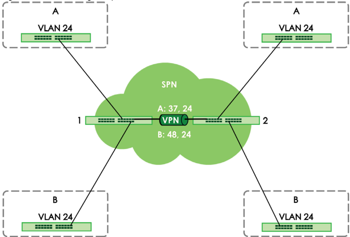
Figure 281 VLAN Stacking Example
