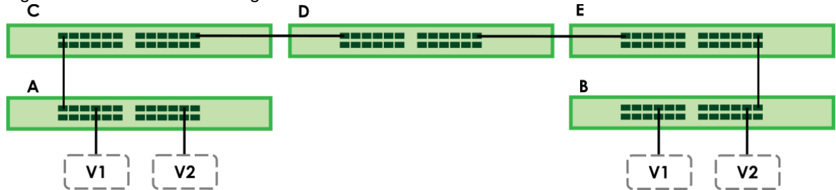
Figure 252 Port VLAN Trunking
