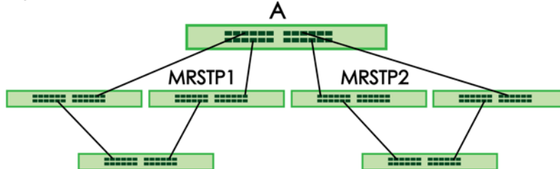
Figure 233 MRSTP Network Example
