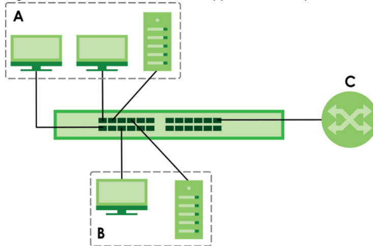
Figure 262 Protocol Based VLAN Application Example
