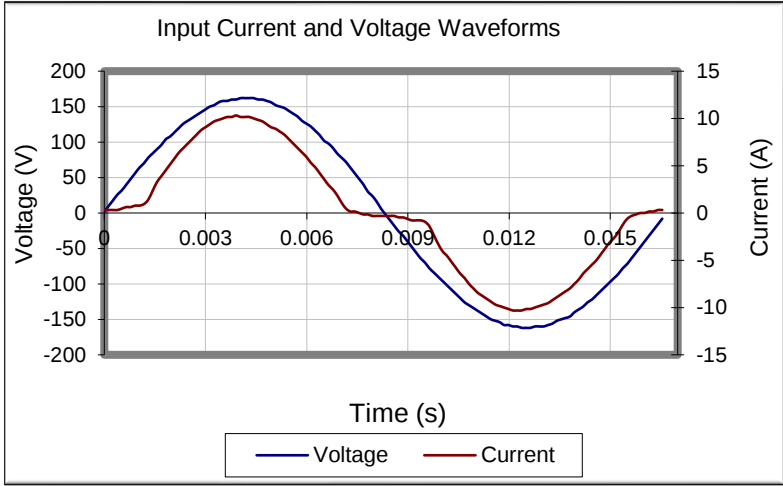
Input AC Current Waveform (ITHD = 30.55%, 50% Load)
