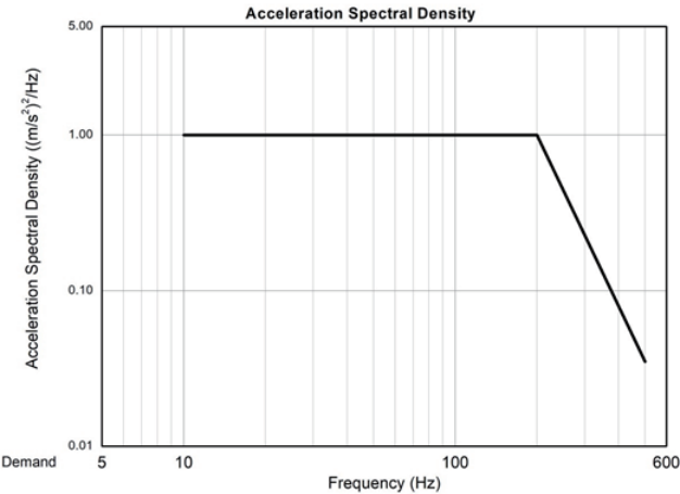
Figure 9-2 – Acceleration Spectral Density
