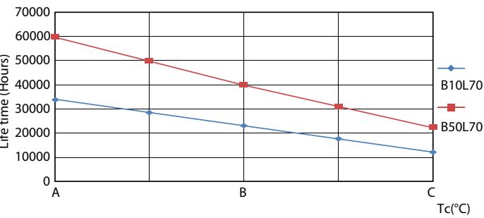
LEDtube_60K_LifetimeVsTc
