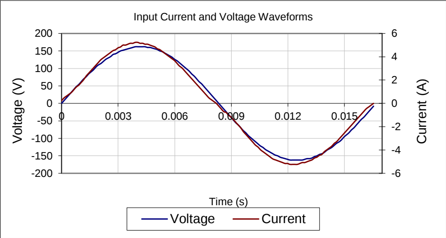
Input AC Current Waveform (ITHD = 4.9%, 50% Load)
