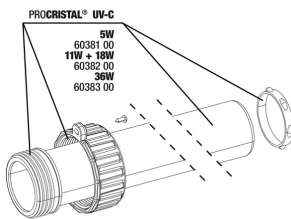
JBL ProCristal UV-C Set Quarzglaskolben
