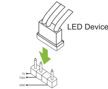
Addressable RGB LED Device Header (5V_LED)
