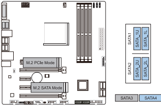
1x M.2 PCIe SSD Slot + 1x M.2 SATA SSD Slot-- 5x SATA HDDs
