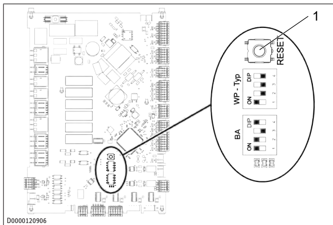
1 Reset-Taster
