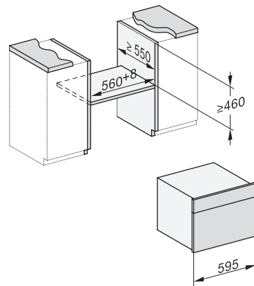
DG7x4x, DGM7x4x, DGC7x4x, DGC7x4xX, DGC7x4xHCPro, DGC7x4xHCXPro Skizze
