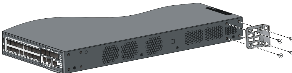
Figure 19 1U mounting bracket rear mounting position
