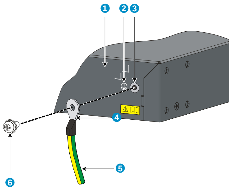
Figure 22 Connect the grounding cable to the grounding hole of switch
