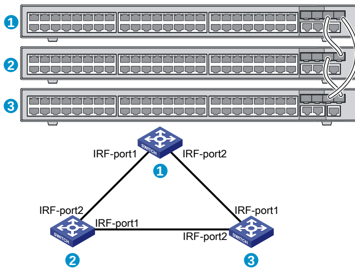
Figure 38 IRF fabric in ring topology
