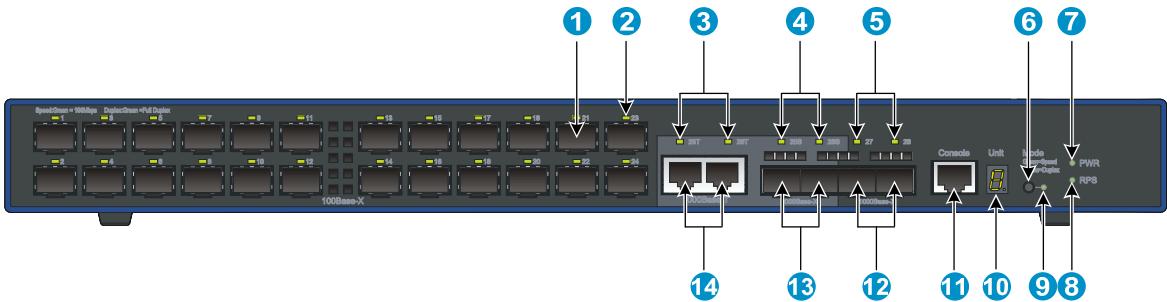
Figure 13 3600-24-SFP v2 EI front panel
