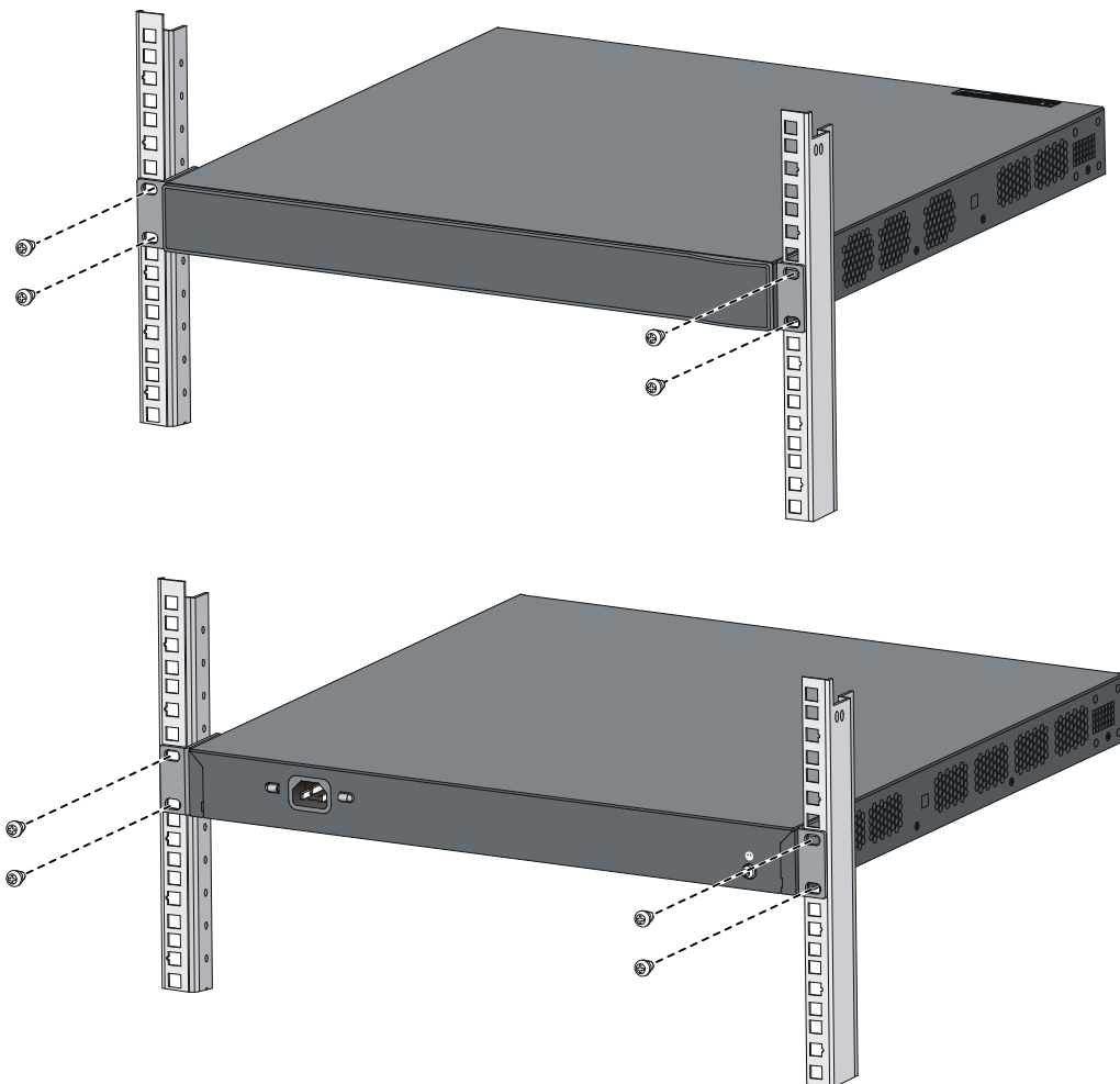
Figure 20 Mount an 3600 v2 switch in a rack
