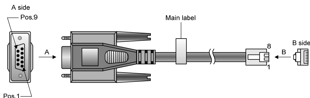
Figure 30 Console cable
