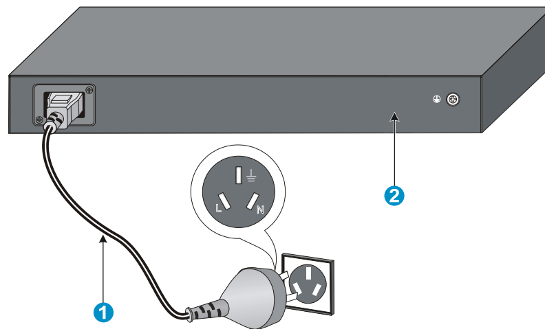
Figure 25 Ground through the PE wire of the AC power supply
