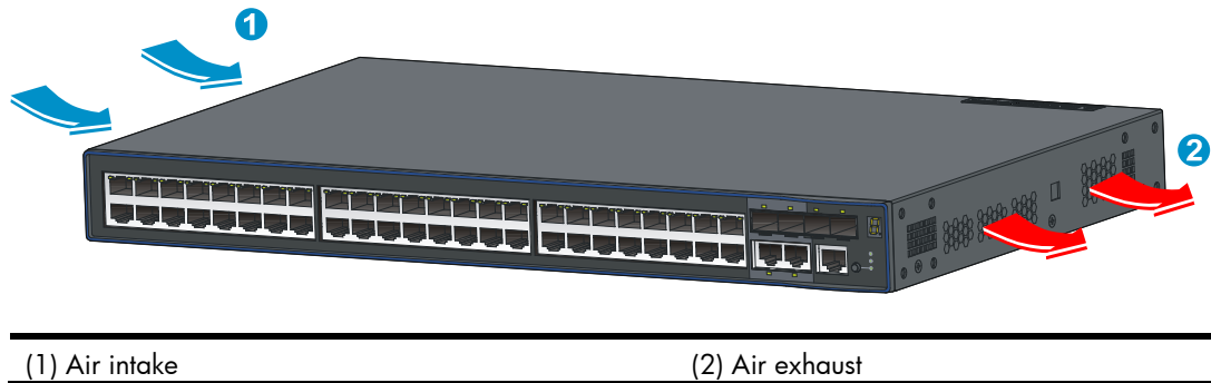
Figure 15 Airflow through the 3600 v2 switches
