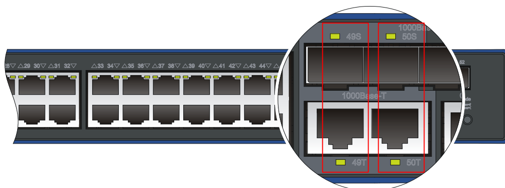
Figure 42 Identify the combo ports on the 3600-48 v2 SI Switch front panel
