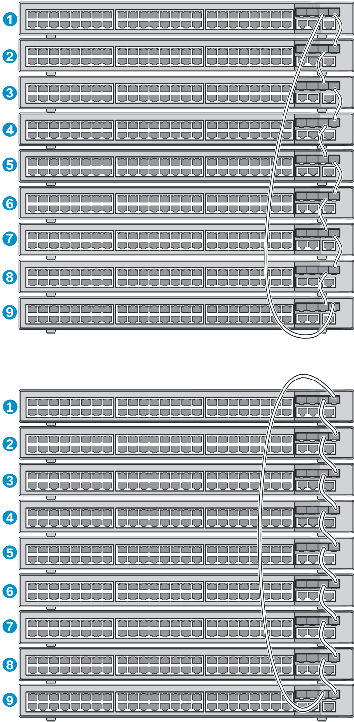
Figure 39 Connect the IRF member switches in one rack
