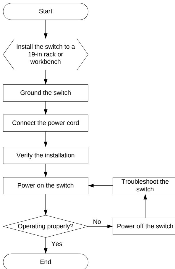
Figure 16 Hardware installation flow
