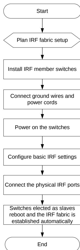
Figure 36 IRF fabric setup flowchart
