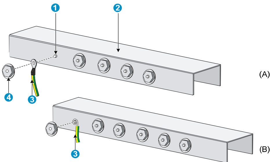
Figure 24 Connect the grounding cable to a grounding strip
