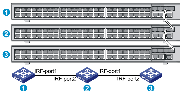
Figure 37 IRF fabric in daisy chain topology
