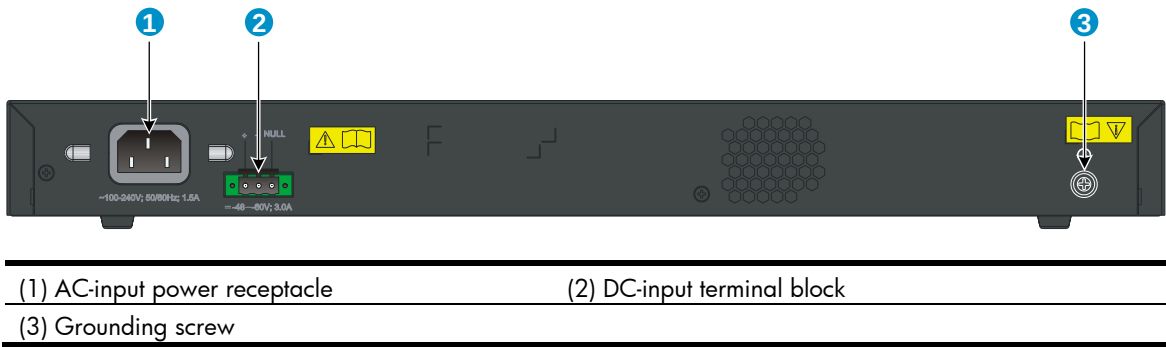
Figure 2 3600-24 v2 EI rear panel
