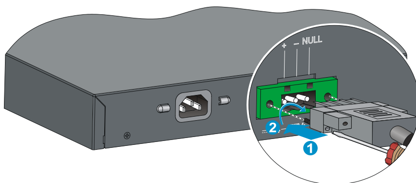
Figure 28 Connect a DC power cord to the switch
