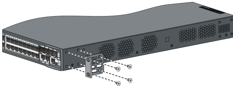
Figure 18 1U mounting bracket front mounting position
