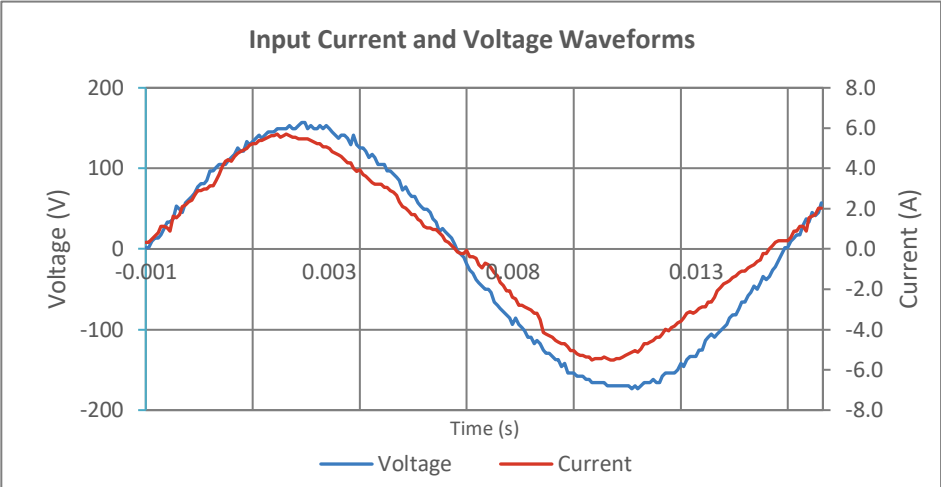
Input AC Current Waveform (ITHD = 9.32%, 50% Load)
