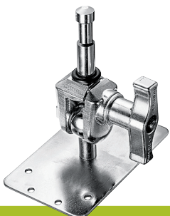
F810 BABY PLATE WITH 16MM SWIVEL SPIGOT
