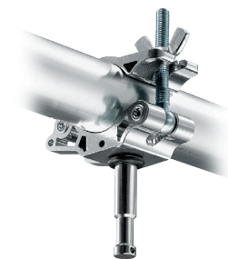
C462-1 LP EYE COUPLER WITH 16MM SPIGOT
