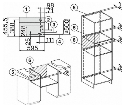
DGC7x45, Skizze
