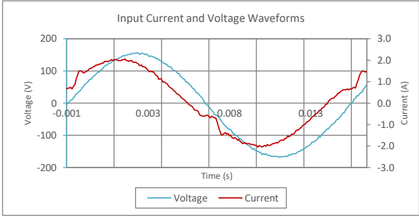
Input AC Current Waveform (ITHD = 6.19%, 50% Load)
