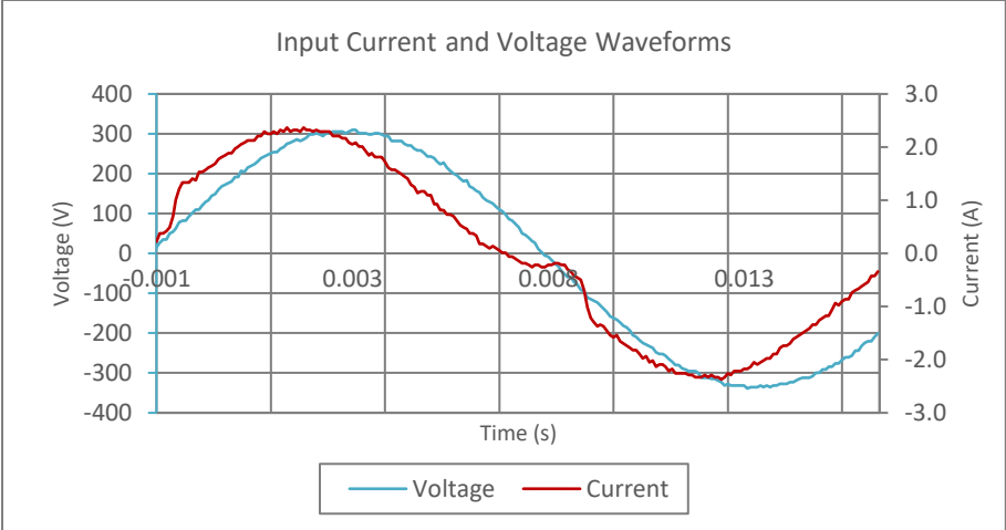
Input AC Current Waveform (ITHD = 14.76%, 50% Load)
