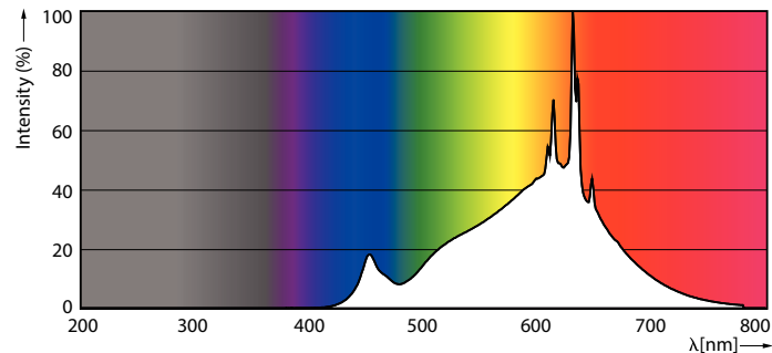
LEDspots MAS 5,8W MR16 GU5,3 927 60D
