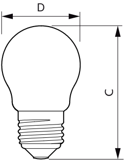
P45 230V 4-25W 250lm 2700-2200K E27 D CL
