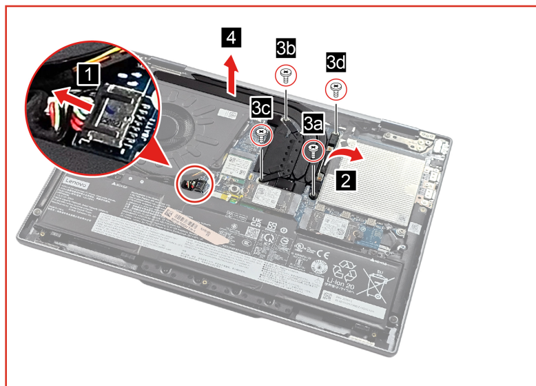
Figure 15. Remove the heat sink (for Intel models)
