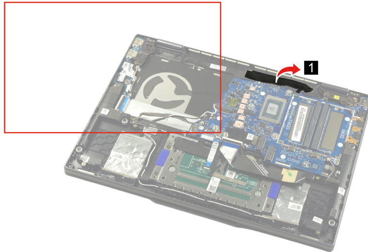
Figure 39. Peel off the MB acetate tape
