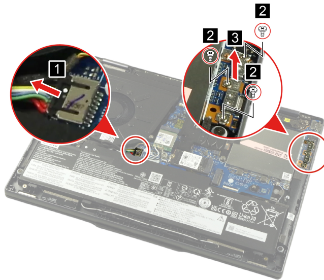
Figure 11. Remove the Type-C bracket
