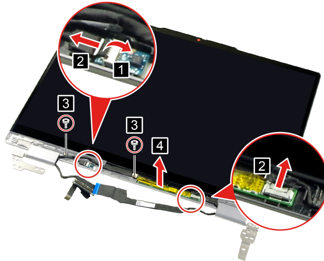
Figure 29. Disconnect the touch board connector and the sensor board connector, remove two screws, and pry up the touch board
