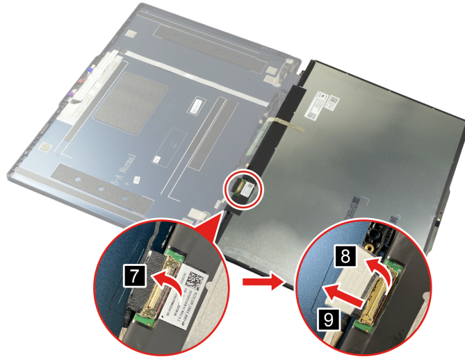
Figure 73. Disconnect the EDP cable
