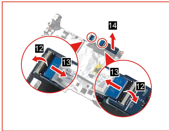
Figure 44. Disconnect the PMIC cable and then remove the PMIC board
