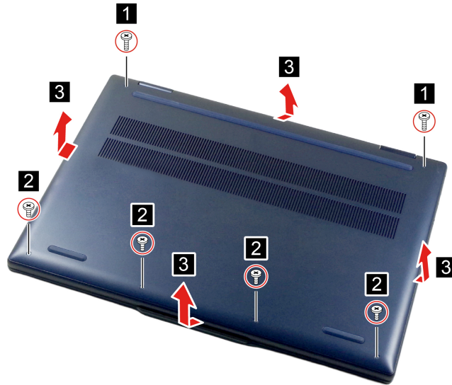
Figure 45. Remove six screws and the lower case
