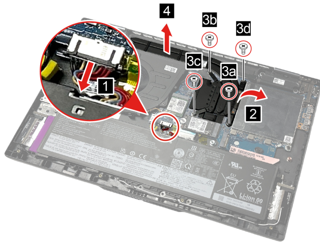
Figure 60. Remove the heat sink (for Intel models) Table 36. Screw used to secure the heat sink (for Intel models)
