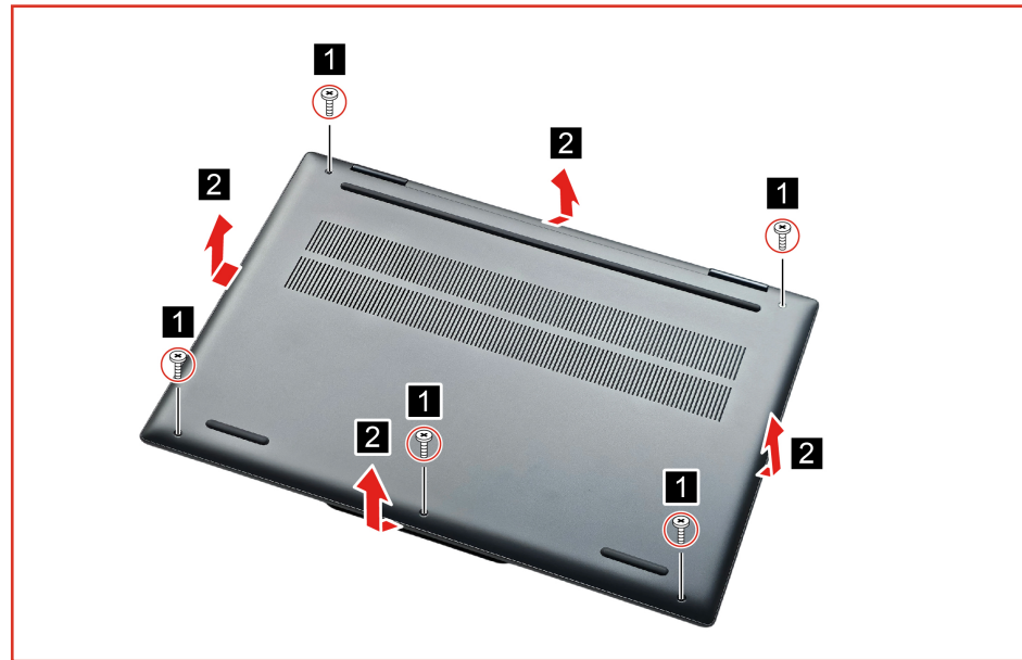
Figure 2. Remove five screws and the lower case (for selected models)
