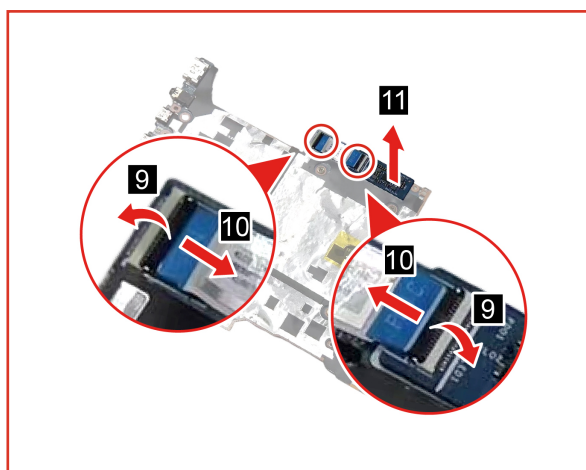
Figure 87. Disconnect the PMIC cable and then remove the PMIC board
