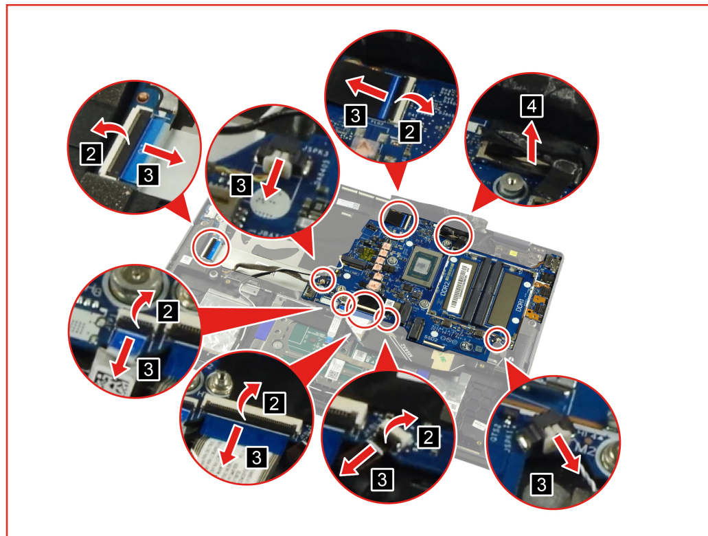
Figure 40. Disconnect the cables
