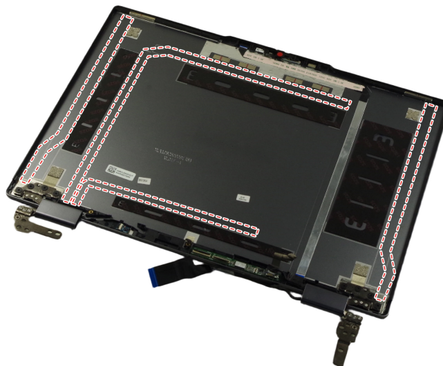
Figure 32. The locations of the stretch-release tapes
