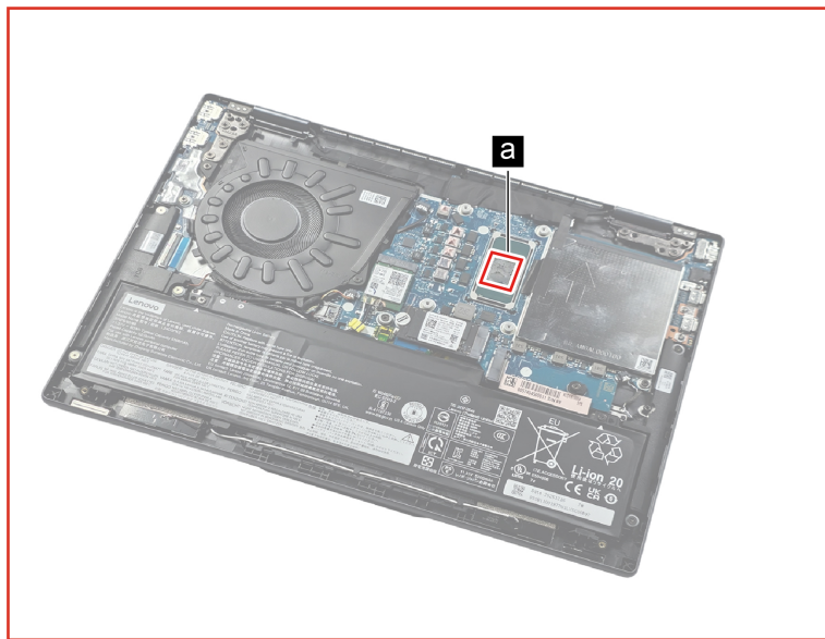
Figure 19. Areas on the system board where thermal interface materials are applied (for Intel models)
