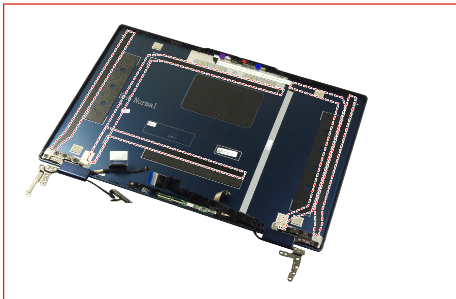
Figure 74. The locations of the stretch-release tapes
