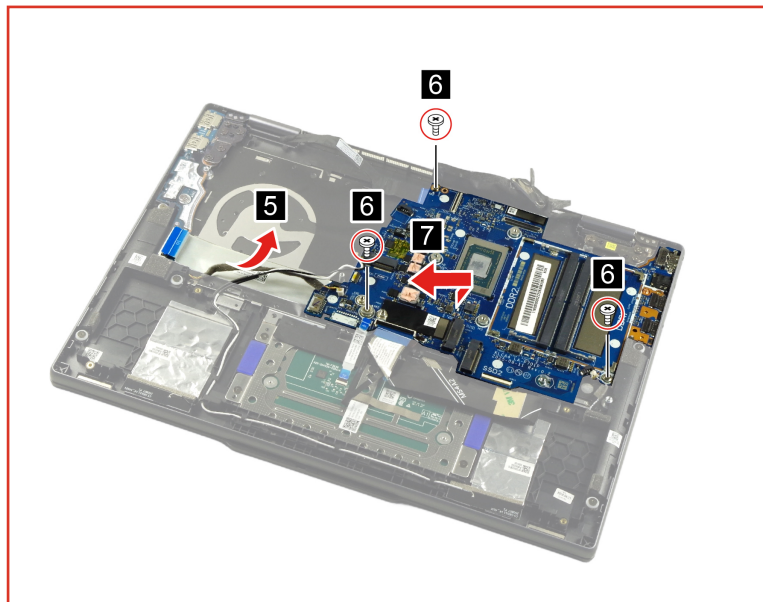
Figure 41. Remove three screws and remove the system board
