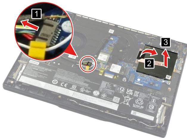
Figure 56. Remove the memory shielding
