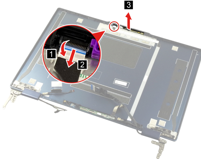
Figure 80. Remove the camera board
