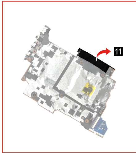
Figure 43. Peel off the MB acetate tape covering the PMIC board and the PMIC cable
