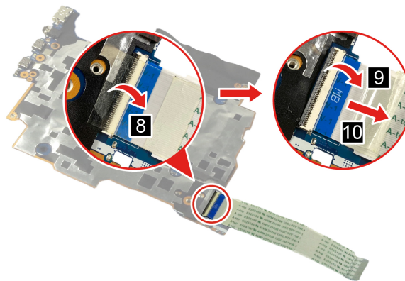
Figure 42. Disconnect the I/O board cable from the system board
