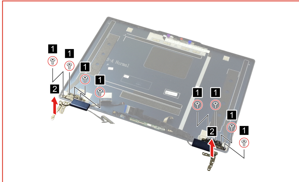
Figure 78. Remove the hinges
