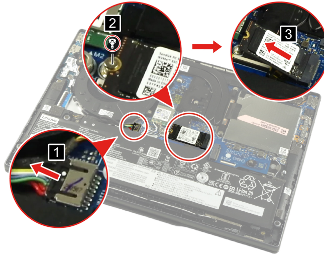
Figure 7. Remove the solid-state drive
