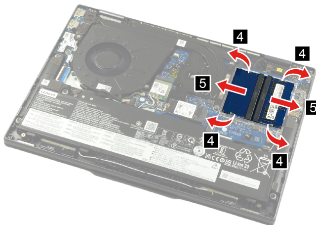
Figure 13. Remove the memory module
