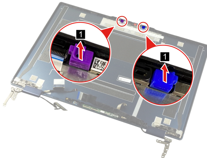
Figure 75. Remove the microphone rubbers
