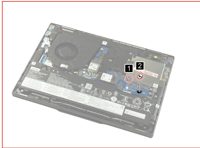
Figure 8. Remove the 2242 trans cover
