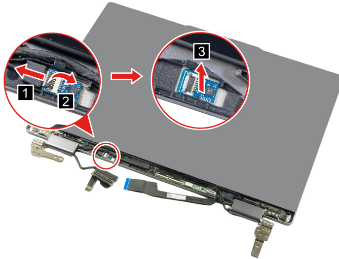
Figure 28. Remove the sensor board
