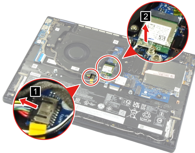
Figure 54. Remove the Wi-Fi card mylar
