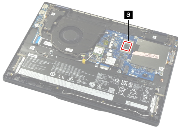
Figure 63. Areas on the system board where thermal interface materials are applied (for AMD models)
