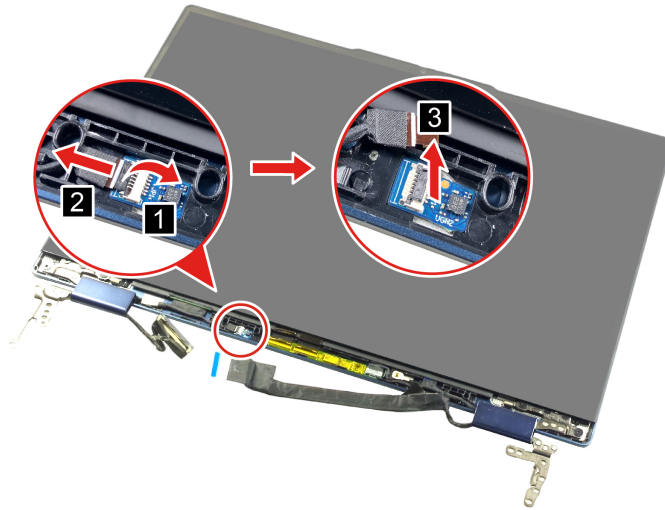
Figure 71. Remove the sensor board
