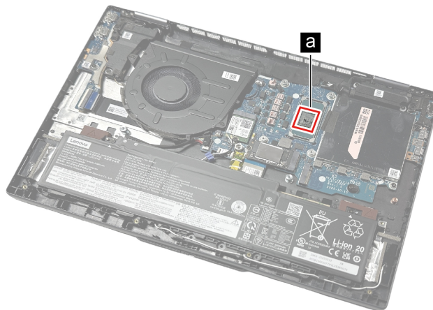
Figure 64. Areas on the system board where thermal interface materials are applied (for Intel models)
