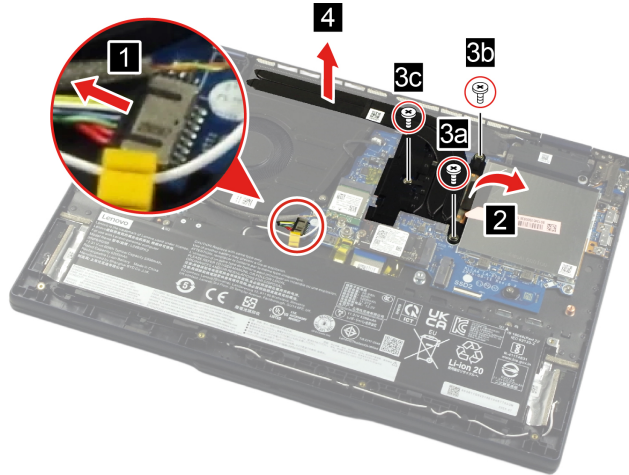
Figure 59. Remove the heat sink (for AMD models) Table 35. Screw used to secure the heat sink (for AMD models)
