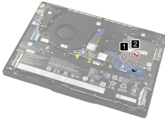
Figure 53. Remove the 2242 trans cover
