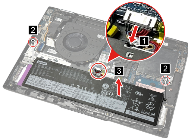
Figure 50. Remove the battery pack (for the 84 Wh battery pack)
