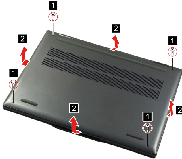
Figure 1. Remove four screws and the lower case (for selected models)
