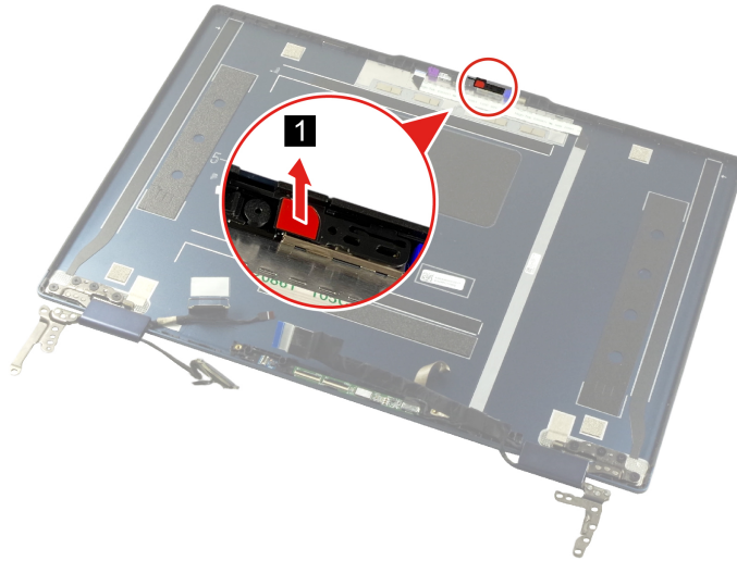
Figure 77. Remove the camera shutter
