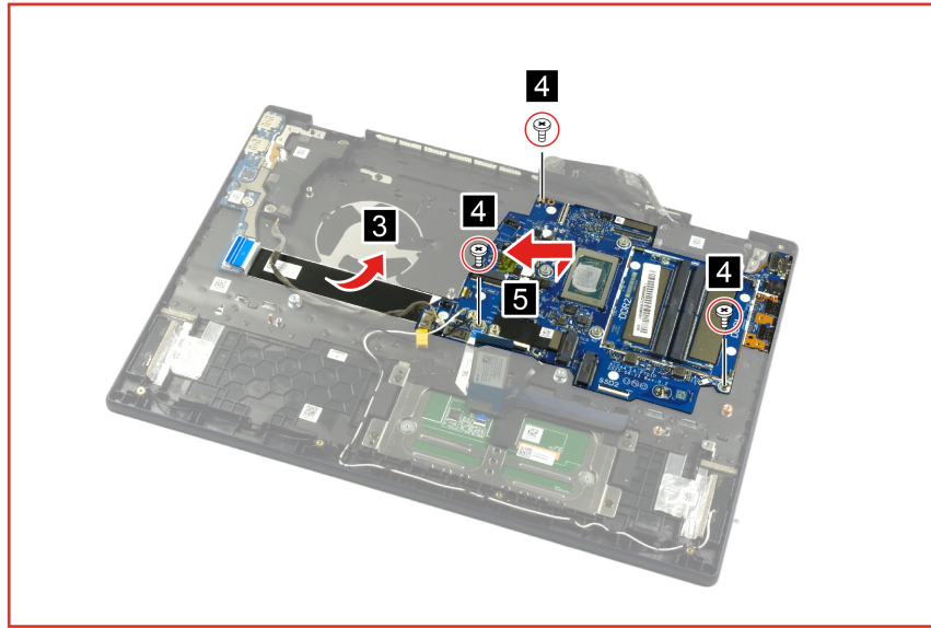
Figure 84. Remove three screws and remove the system board
