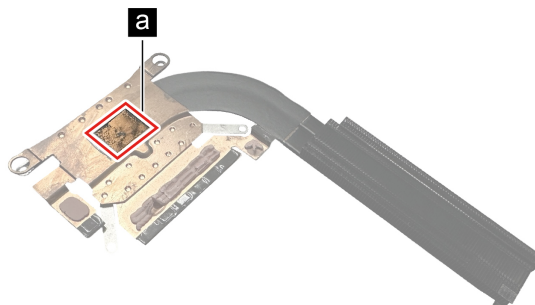
Figure 62. Areas on the heat sink where thermal interface materials should be applied (for Intel models)
