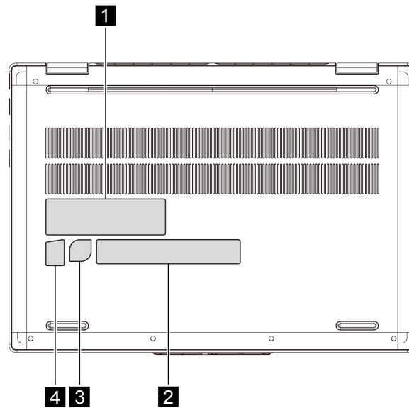
Figure 48. Label layout on the back side of the lower case (for non-EAA countries or regions)
