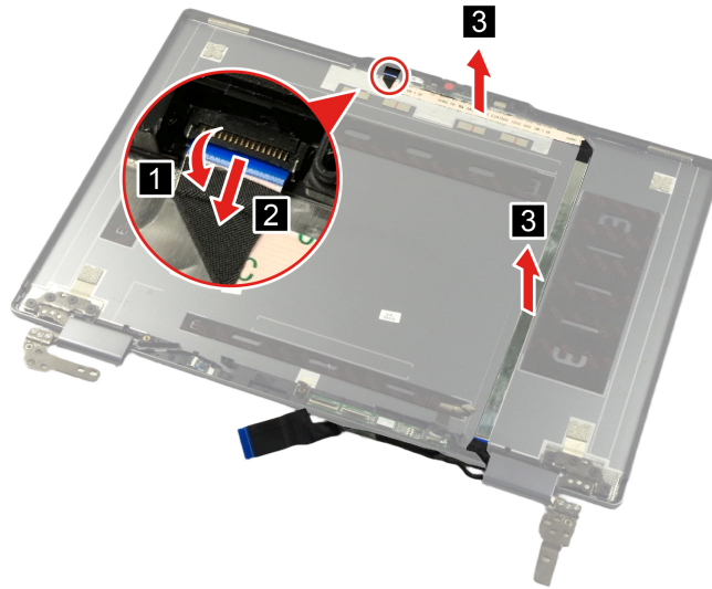
Figure 37. Remove the camera cable
