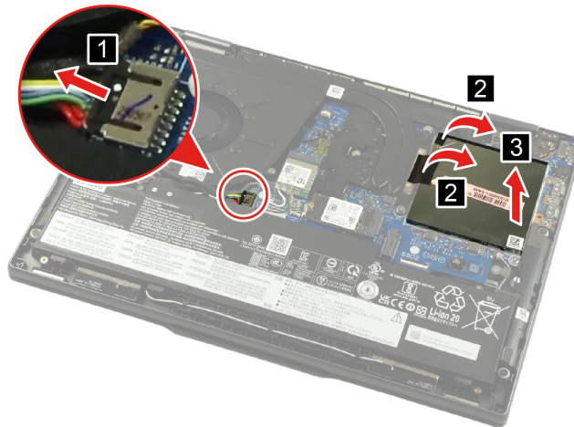
Figure 12. Remove the memory shielding
