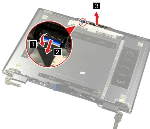
Figure 38. Remove the camera board
