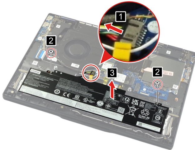
Figure 49. Remove the battery pack (for the 60 Wh battery pack)
