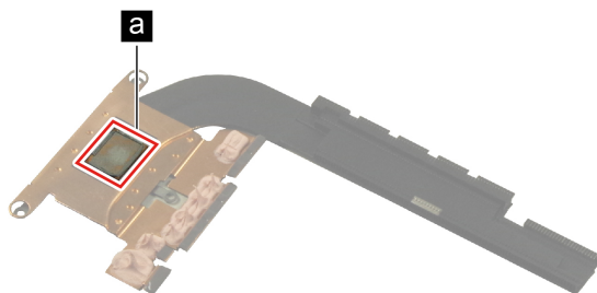
Figure 16. Areas on the heat sink where thermal interface materials should be applied (for AMD models)
