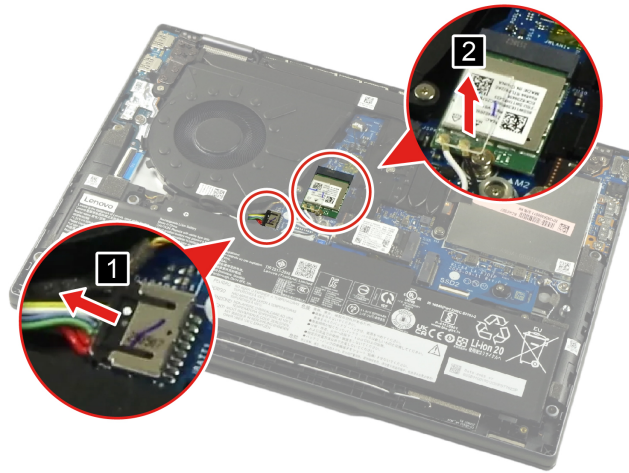
Figure 9. Remove the Wi-Fi card mylar
