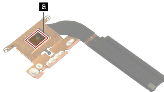
Figure 61. Areas on the heat sink where thermal interface materials should be applied (for AMD models)
