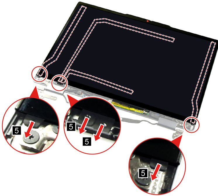
Figure 30. Take out the stretch-release tapes
