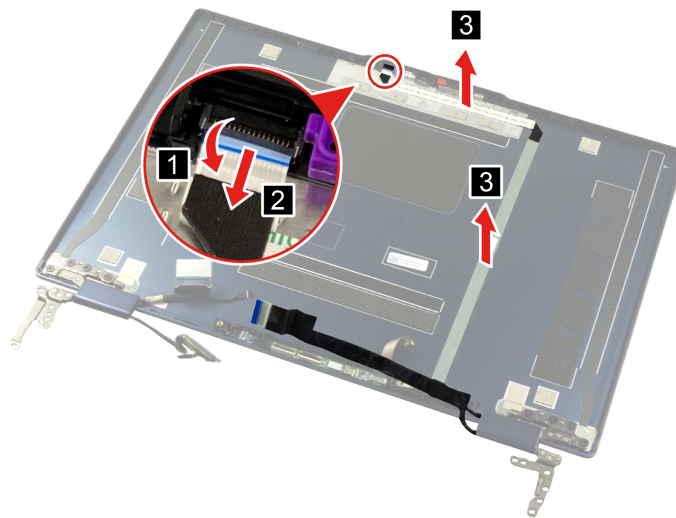
Figure 79. Remove the camera cable
