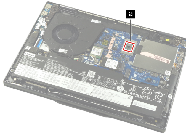
Figure 18. Areas on the system board where thermal interface materials are applied (for AMD models)
