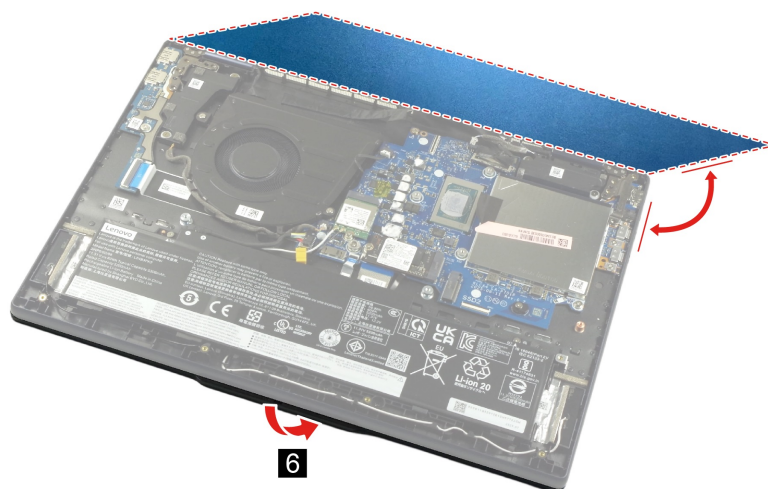
Figure 69. Remove the display module
