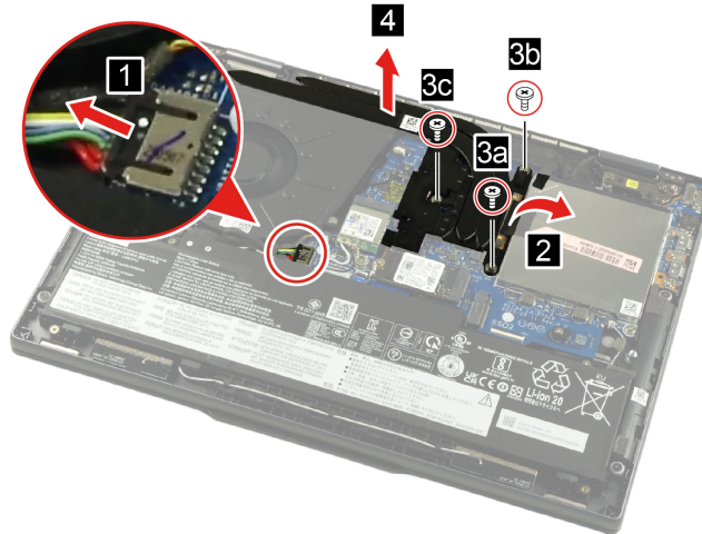
Figure 14. Remove the heat sink (for AMD models)
