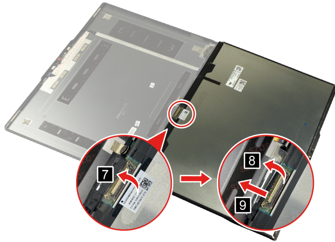
Figure 31. Remove the EDP cable
