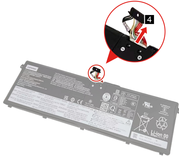
Figure 51. Remove the battery pack cable of the 84 Wh battery pack
