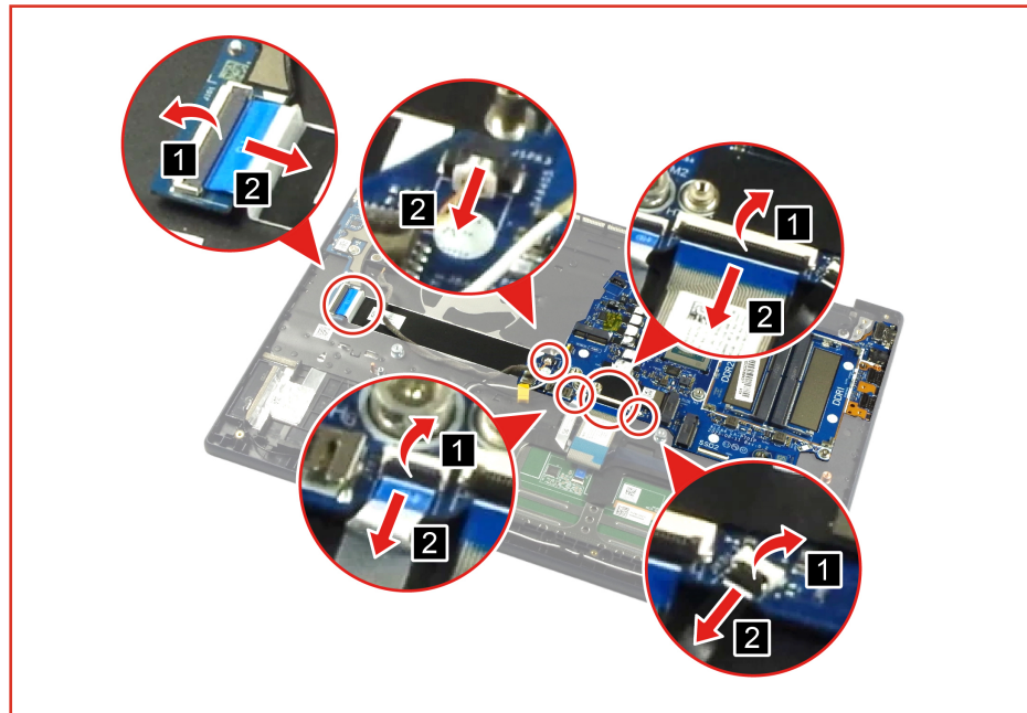
Figure 83. Disconnect the cables
