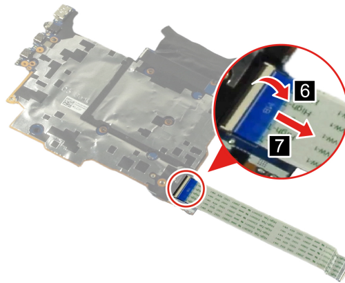
Figure 85. Disconnect the I/O board cable from the system board
