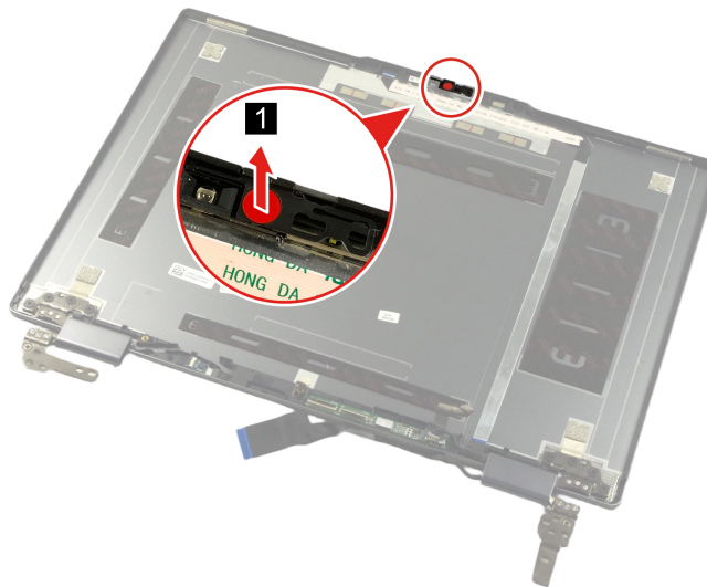
Figure 36. Remove the camera shutter
