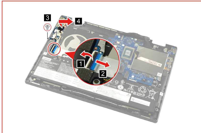
Figure 22. Remove the I/O board
