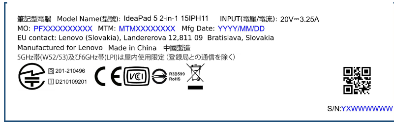
Figure 139. Artworks for the laser etched label used in Japan
