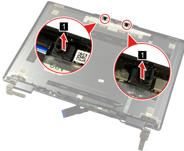
Figure 34. Remove the microphone rubbers
