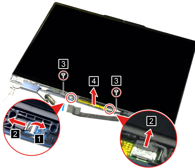
Figure 72. Disconnect the touch board connector and the sensor board connector, remove two screws, and pry up the touch board
