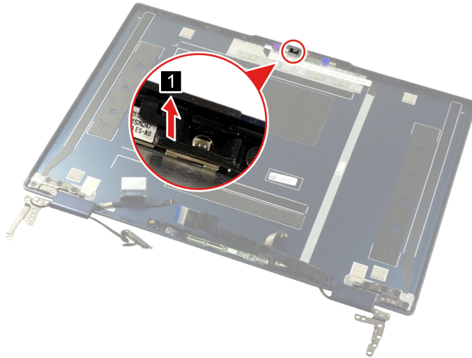
Figure 76. Remove the IR rubber
