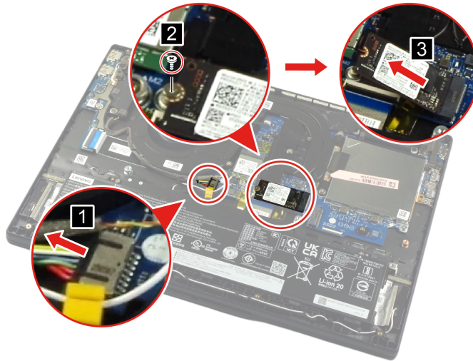
Figure 52. Remove the solid-state drive
