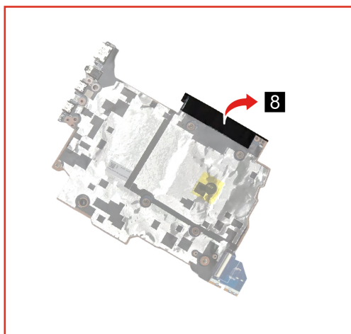
Figure 86. Peel off the MB acetate tape covering the PMIC board and the PMIC cable
