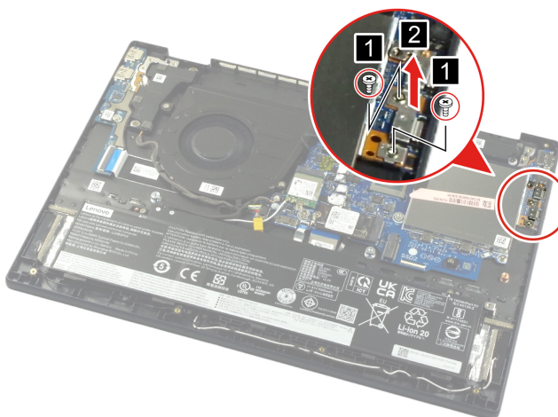
Figure 81. Remove the Type-C bracket
