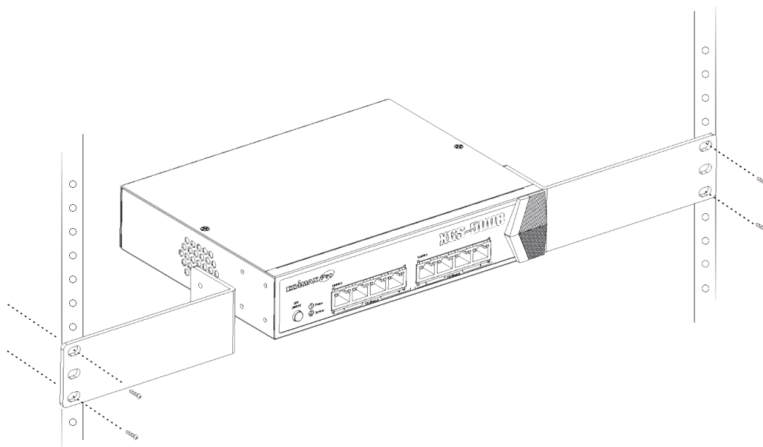
Rack-mount Installation
