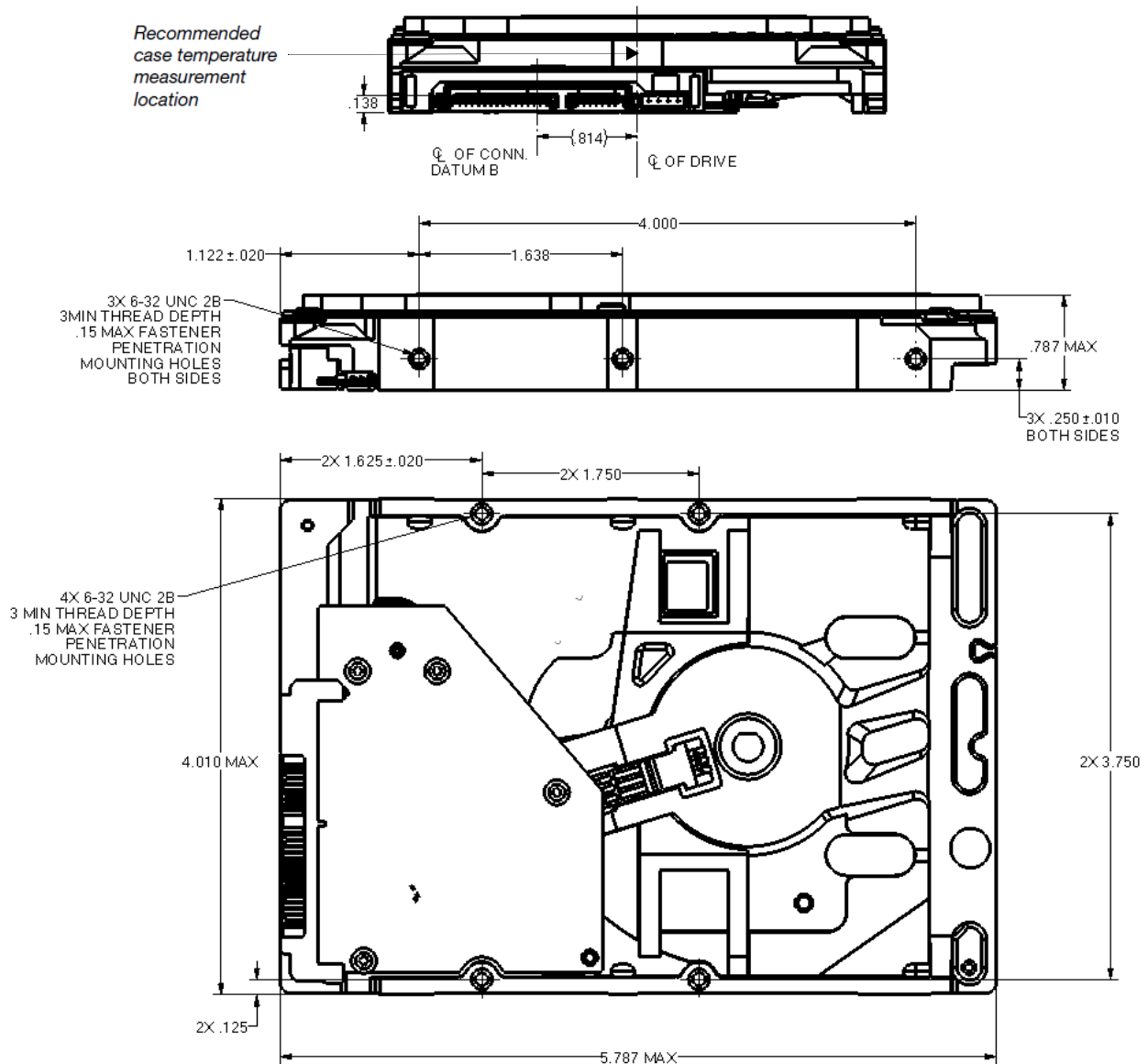
Figure 4 Mounting dimensions (1TB and 500GB models)
