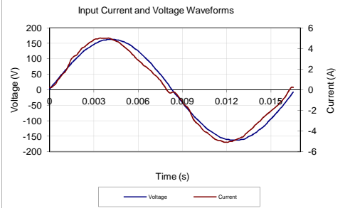
Input AC Current Waveform (ITHD = 8.93%, 50% Load)
