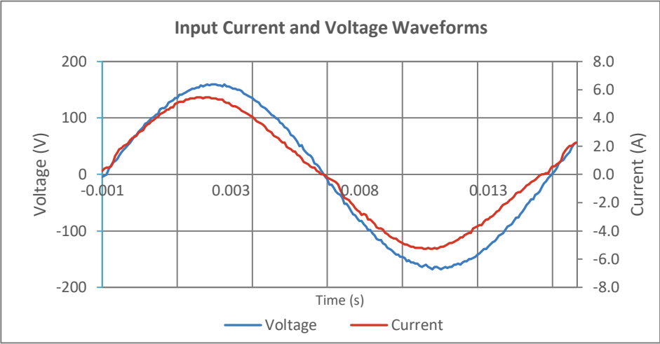
Input AC Current Waveform (ITHD = 6.03%, 50% Load)
