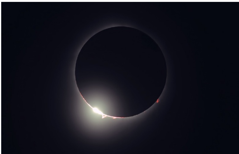
The April 2024 total solar eclipse observed with Vespera. (post-processed image)
