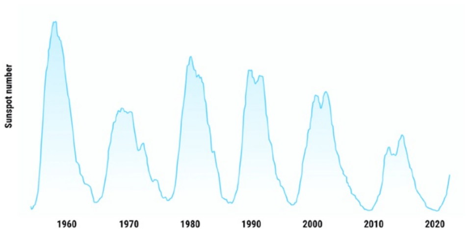
Evolution of solar activity over the years
