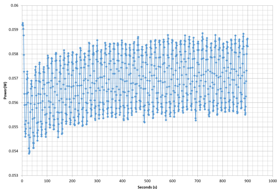
Power - R1701TA101450009 - 12/10/2017 - 16:14
