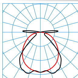
OleveonF 6 B 2000-840 PC +LV TX372198
