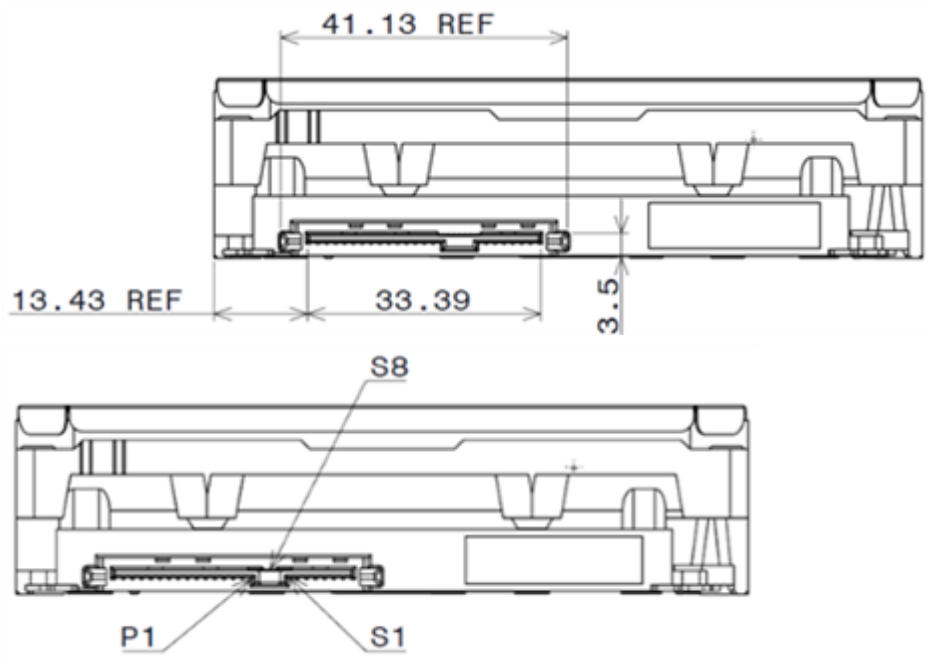
Figure 9 Connector locations
