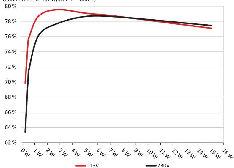
5VSB Efficiency: Thermaltake Toughpower GF1 1000W
