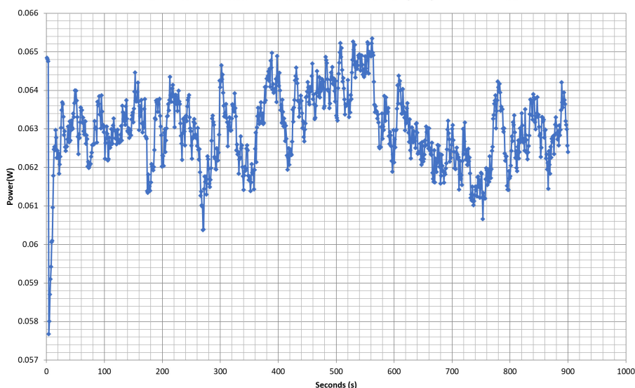
Power - PSTPD1000FNFAGU1XU000245 - 31/07/2021 - 12:59
