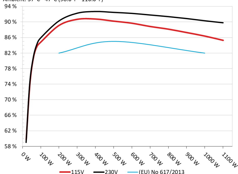
Efficiency: Thermaltake Toughpower GF1 1000W
