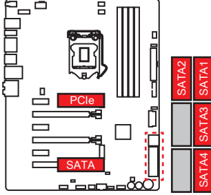
1xM.2 SATA SSD + 1xM.2 PCIe SSD + 4xSATA HDDs
