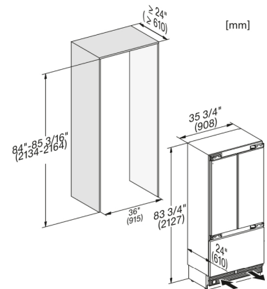
KF2982Vi, KF2981Vi, Installation, MasterCool, Skizze
