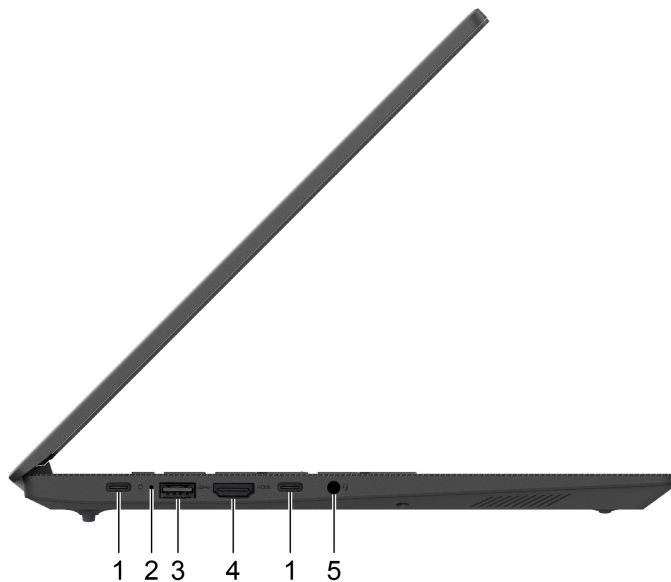
Figure 10: Lenovo V15 G6 AMN—left-side view
