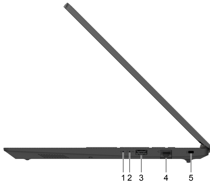
Figure 16: Lenovo V15 G6 AMN—right-side view
