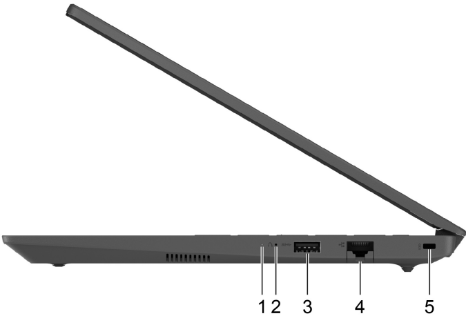
Figure 11: Lenovo V14 G6 ITN—right-side view
