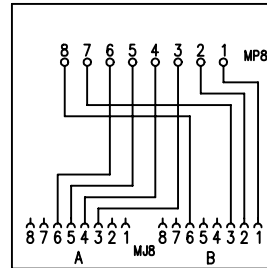
T-Adapter Cat.5 ISDN / 10/100BT 4-5, 3-6/1-2, 3-6
