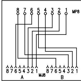
T-Adapter Cat.5 10/100BT / 10/100BT 1-2, 3-6/1-2, 3-6
