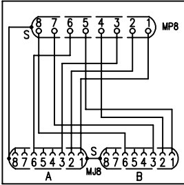
T-Adapter S Cat.5 10/100BT / 10/100BT 1-2, 3-6/1-2, 3-6
