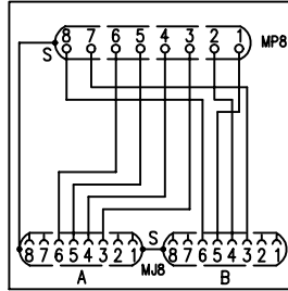
T-Adapter S Cat.5 ISDN,TR / ISDN,TR 4-5, 3-6/4-5, 3-6
