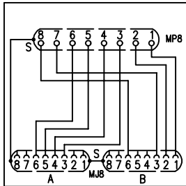
T-Adapter S Cat.5 ISDN / 10/100BT 4-5, 3-6/1-2, 3-6
