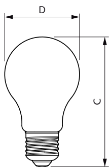
MASTER VLE LEDBulbDT10.5-100W E27 927A60CLG
