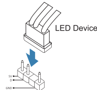
Addressable RGB LED Device Header (5V_LED)
