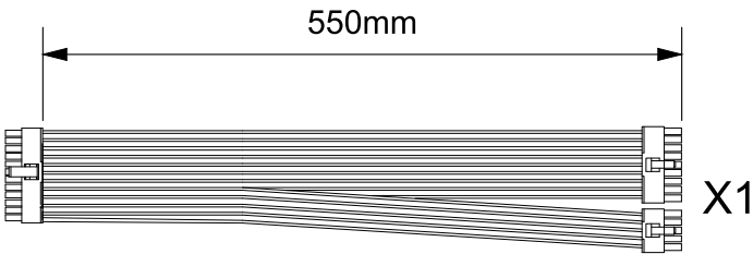
MOTHERBOARD POWER CABLE
