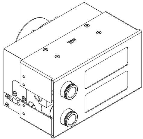
Alphacool ES 2U Reservoir VPP with flow and temperature sensors
