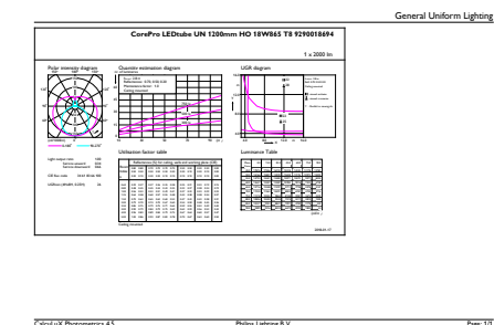
CalcutX Photometrics 4.5 Philips Lighting B.V. Page 1/1
