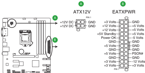
B150M-A ATX power connectors
