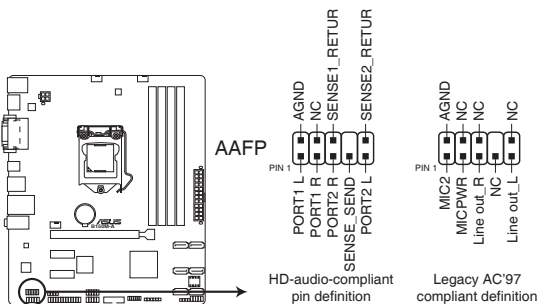
B150M-A Front panel audio connector
