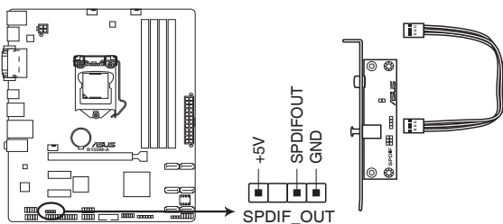
B150M-A Digital audio connector
