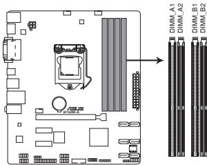
B150M-A 288-pin DDR4 DIMM sockets
