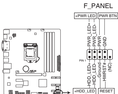
B150M-A System panel connector
