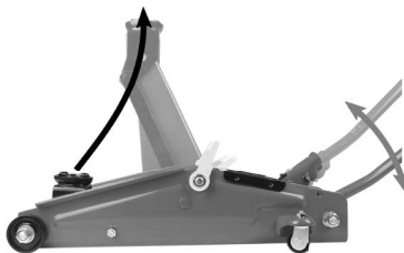
Figure 3: Lifting the vehicle
