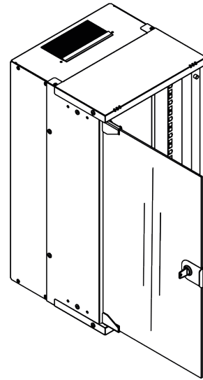
Isometric views
