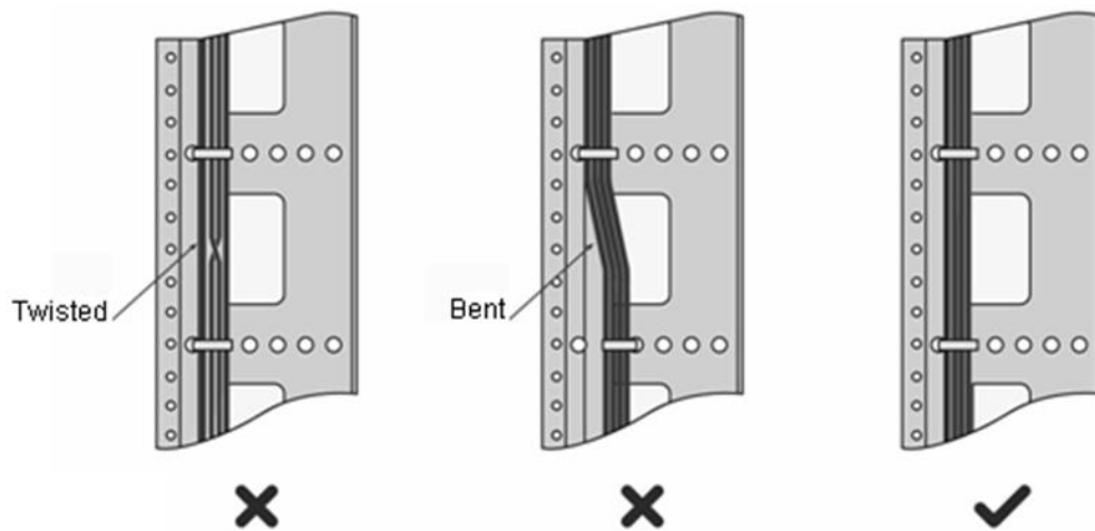
Figure 6-3 Binding Cables (1)
