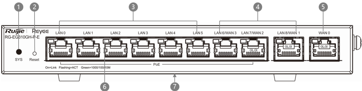
Figure 1-8 Front Panel of an RG-EG310GH-P-E Router
