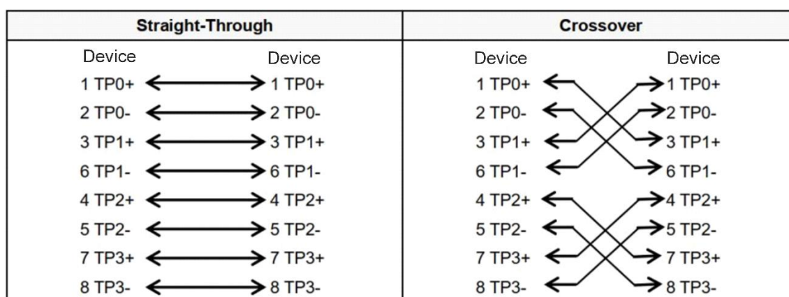
Figure 6-1 1000BASE-T Connection
