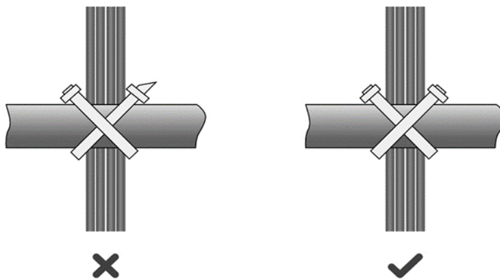
Figure 6-4 Binding Cables (2)
