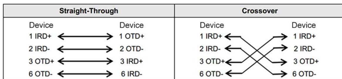
Figure 6-2 100BASE-TX/10BASE-T Connection
