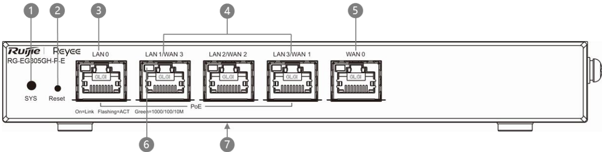
Figure 1-2 Front Panel of an RG-EG305GH-P-E Router
