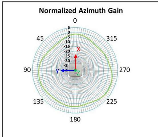
2.4 GHz Azimuth
