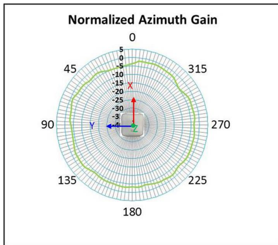
5 GHz Azimuth
