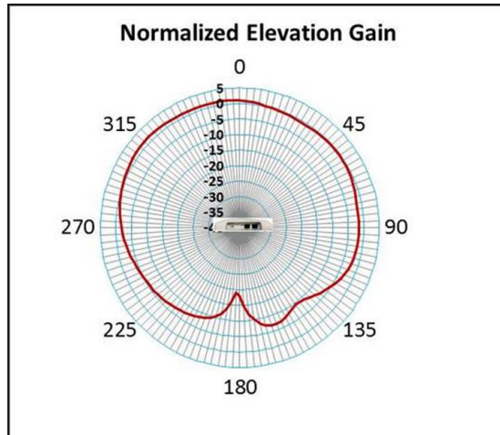
2.4 GHz Elevation
