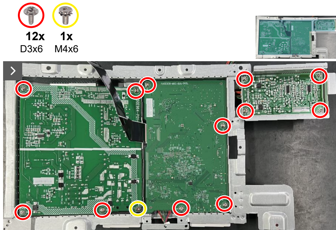
Figure 32. Replace the screws
