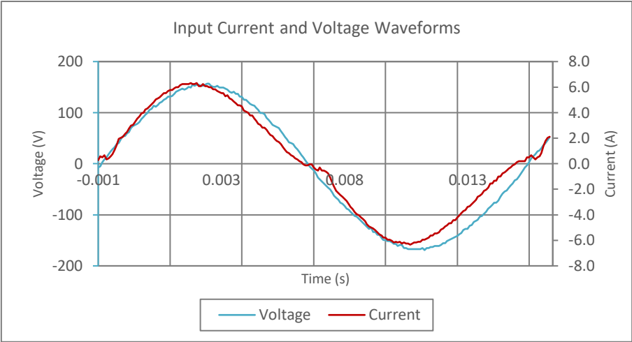
Input AC Current Waveform (ITHD = 10.9%, 50% Load)
