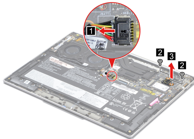
Figure 15. Remove two screws and remove the PMIC board
