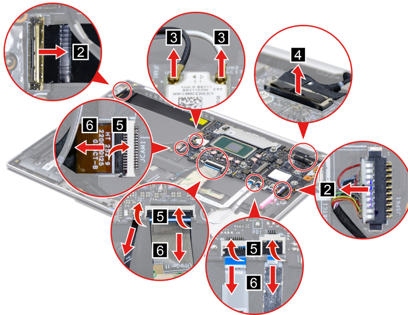
Figure 18. Disconnect cables
